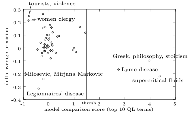
Figure 4: A scatter plot of \Delta average precision and model comparison scores for each of the 50 queries of TREC 8. The \Delta average precision is the value with relevance retrieval(Rel) minus the value with query likelihood retrieval(QL). The model comparison score is the KL divergence from a QL ranked list model to a Rel ranked list model computed over just the top 10 terms in clarity contribution to the QL model. The automatic threshold indicating a score greater than 95% of random one term queries (see Section 4) is shown as a vertical line labeled 'thres' and seven extreme case queries are labelled.
