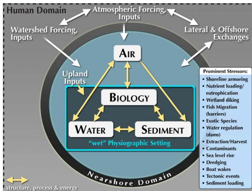
Figure 4. PSNERP-NST Conceptual Model Level 2: Organization of nearshore ecosystem relative to external and internal forcing, structure and processes.
