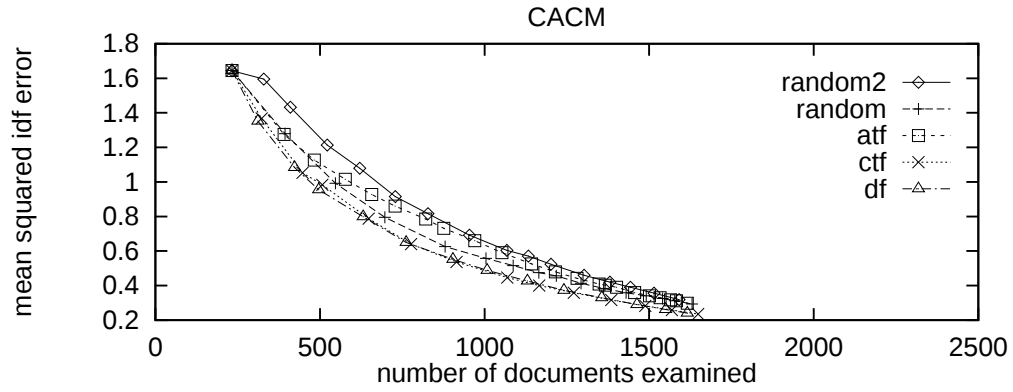
Figure 8: CACM: mean squared idf error
