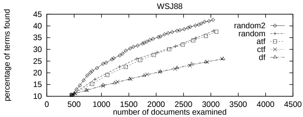
Figure 1: WSJ88: percentage of terms found by probing
