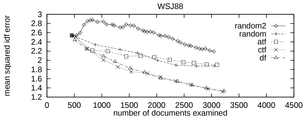
Figure 4: WSJ88: mean squared idf error
