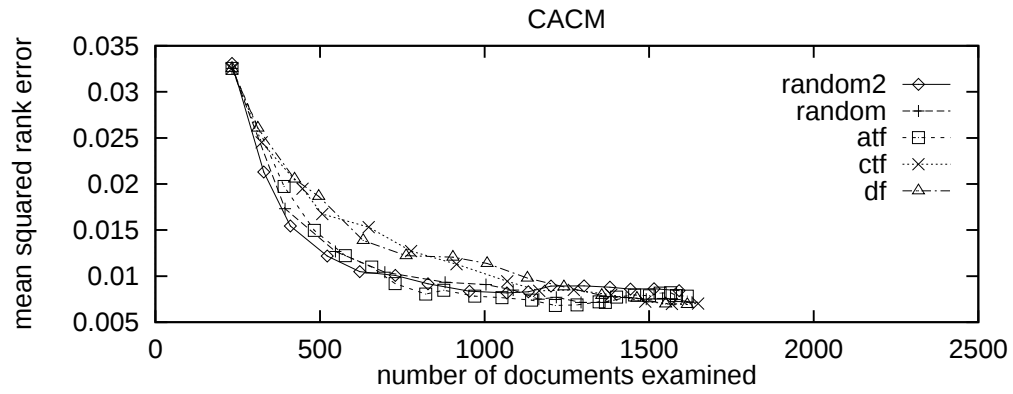
Figure 7: CACM: mean squared rank error
