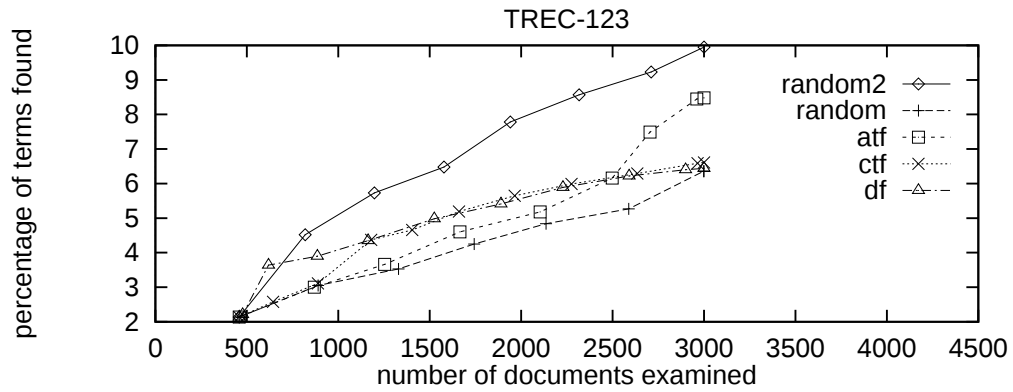
Figure 9: TREC-123: percentage of terms found by probing
