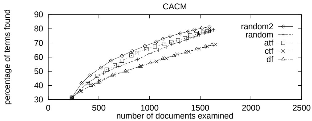
Figure 5: CACM: percentage of terms found by probing
