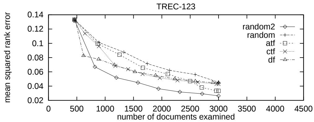
Figure 11: TREC-123: mean squared rank error
