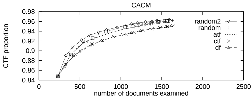
Figure 6: CACM: CTF proportion
