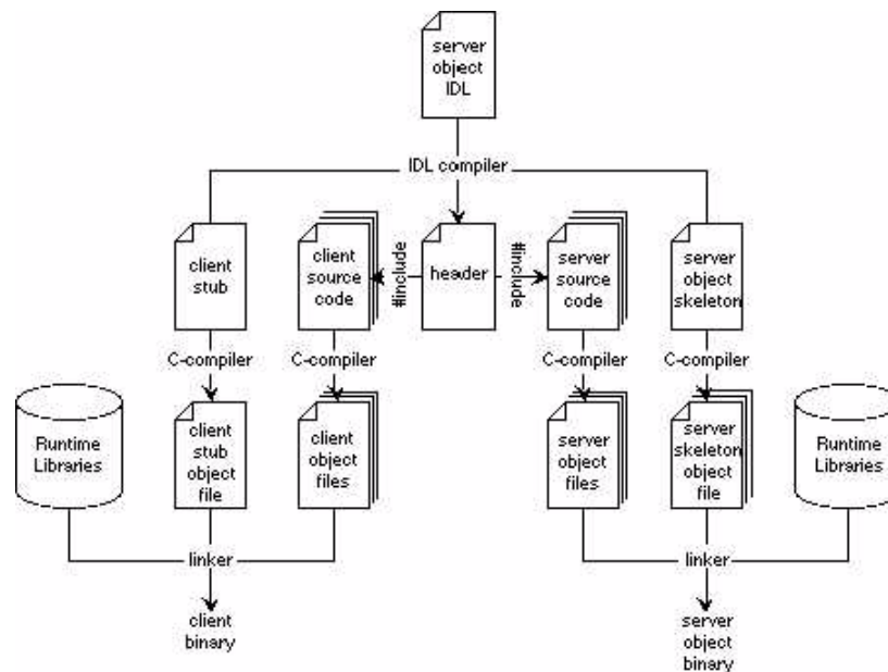
Figure 1 - Process to Implement CORBA Clients and Servers
