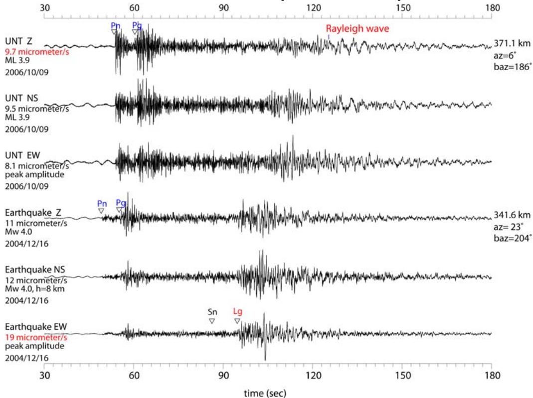
Figure 1. Three-component Records at MDJ (Mudanjiang, NE China) from the Presumed North Korean Nuclear Test on 9 October 2006 (ML 3.9, Shallow) and a Nearby Earthquake on 16 December 2004 (Mw 4.0; h=8km)
