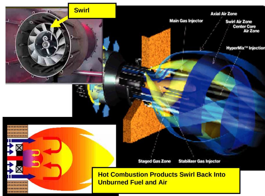
Figure 9. Industry norm swirl stabilized combustion.
