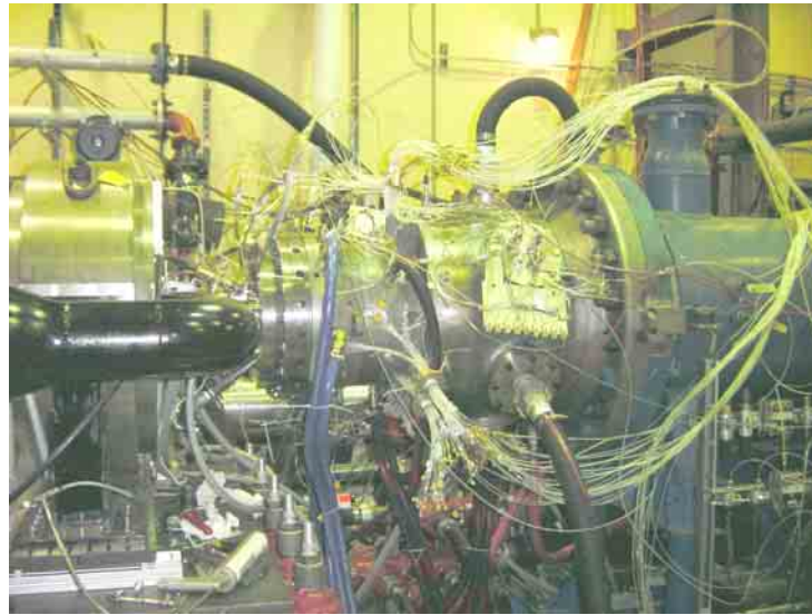
Figure 13. Rampressor-1 test rig installed in test cell.
