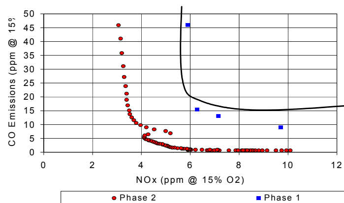
Figure 24. Ramgen AVC extremely low NO x test results.
