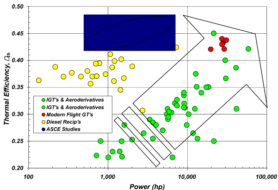
Figure 37. Thermal efficiency vs. rated power.
