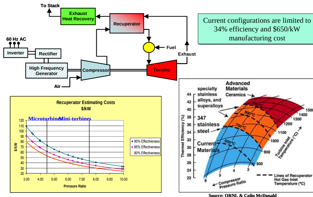
Figure 31. Trade-offs of efficiency gains and recuperator cost.
