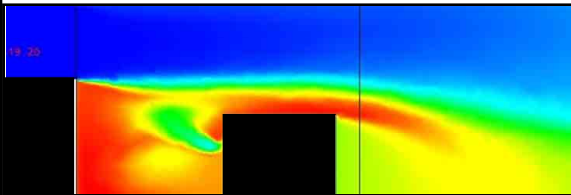
CFD simulation of advanced vortex combustion
