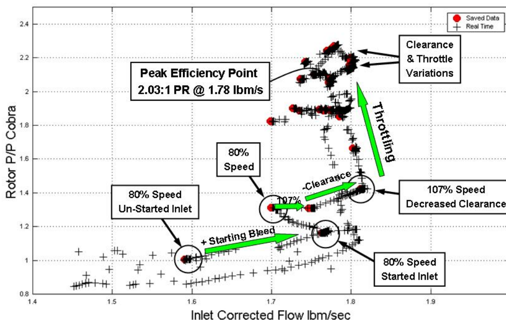
Figure 15. Effect of clearance, bleed, and throttling.
