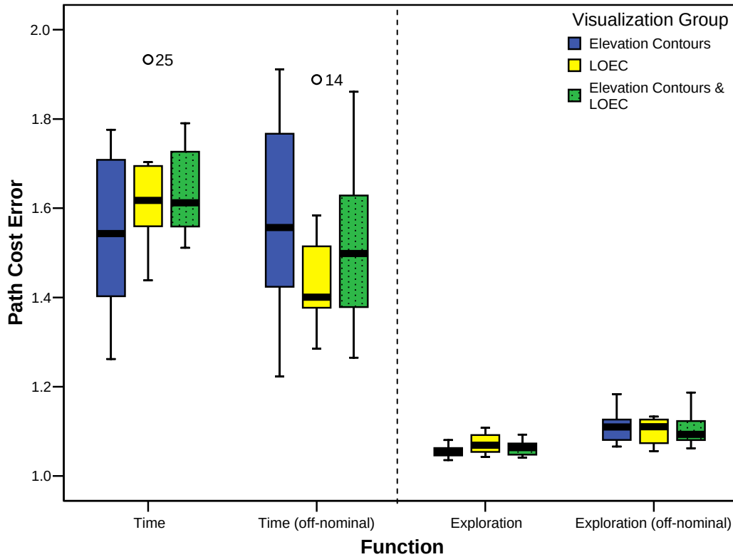
Figure 6.9 Box-plot of path cost errors between visualizations and scenario type, Phase 2
