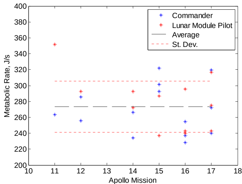
Figure 4.11 Average EVA metabolic rates of astronauts during Apollo missions (data from Waligora and Horrigan, 1975)
