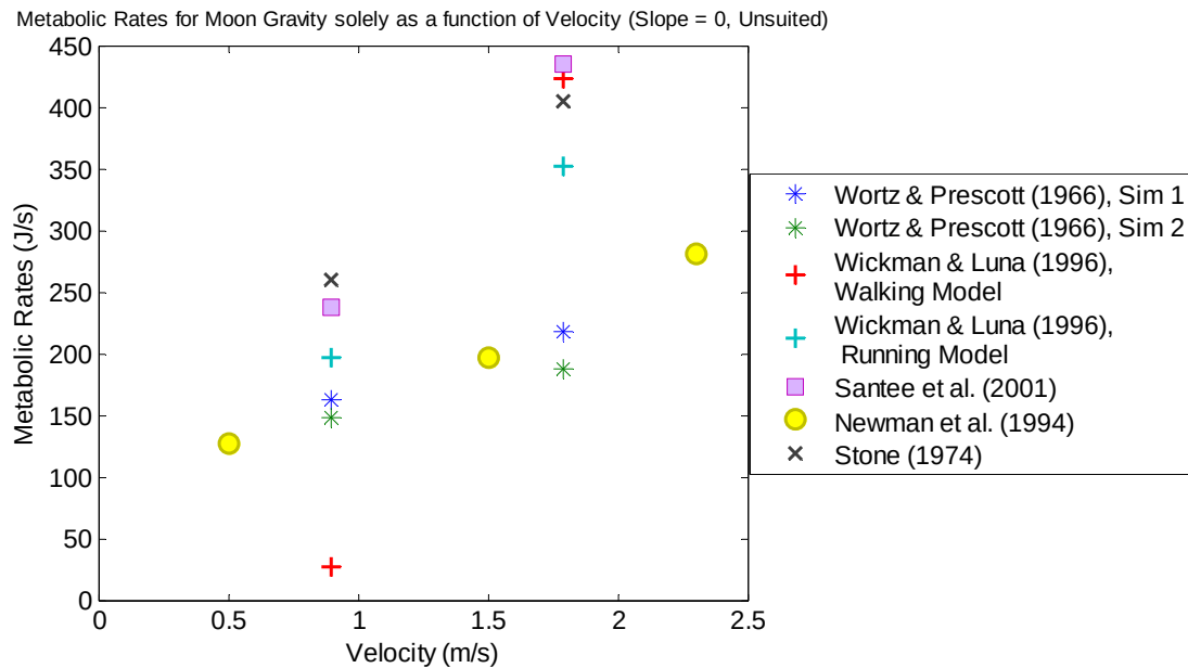
Figure 4.10 Summary of lunar metabolic rates as a function of velocity (on flat terrain)
