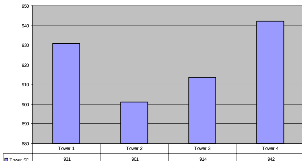
Figure 10. Average conductivity of all cooling towers at Fort Stewart.
