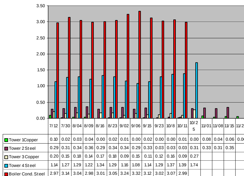
Figure 23. Fort Stewart Corrosion Results.
