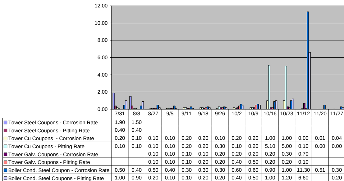
Figure 22. Corrosion results and analyses for cooling towers and condensate at Fort Hood.
