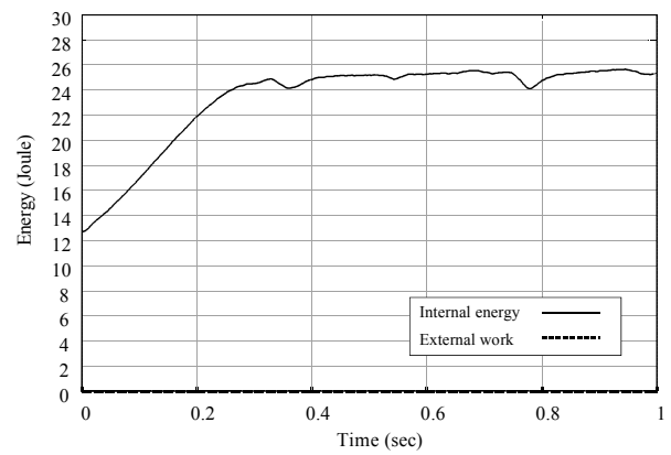
(b) Energy in free expansion process
