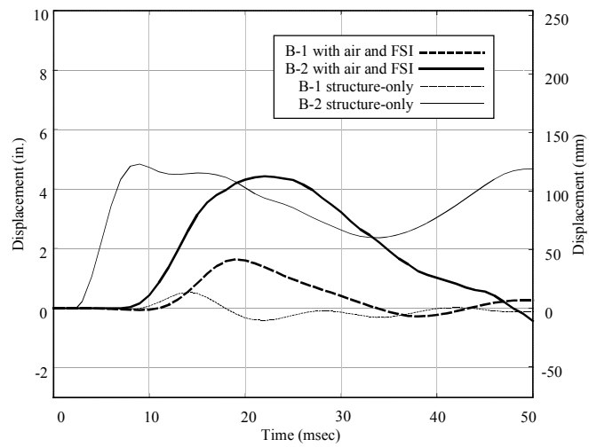
b) Rear panel
