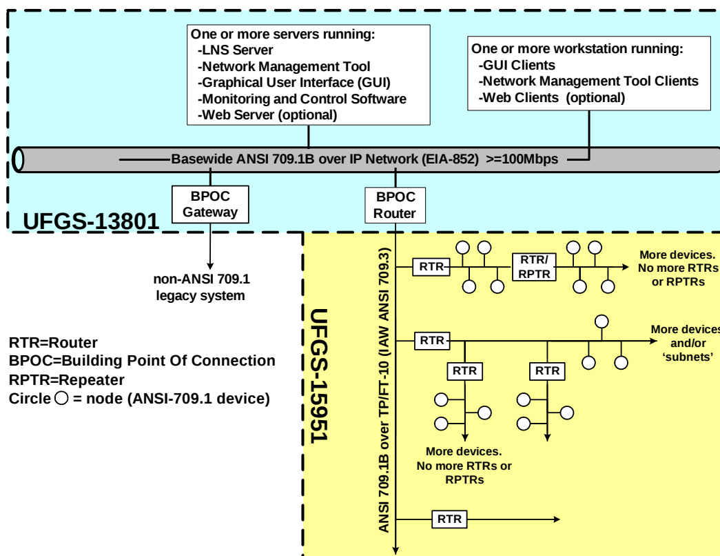
Figure 2. BAS comprised of UMCS and DDC systems.
