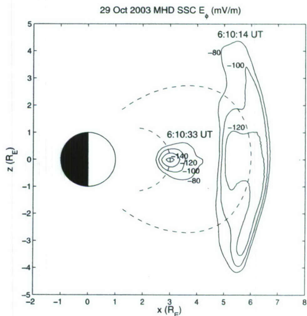
Figure 6. MHD E_\phi peak at 6 R_E and at 3 R_E (two separate time snapshots) on the dayside in the noon-midnight meridional plane in solar magnetic (SM) coordinates. Contours from -80 to -140 mV/m in steps of -20 mV/m are shown. Dashed lines show magnetic field lines through x = 6 R_E and x = 3 R_E traced in the MHD fields in each respective time snapshot.
