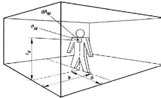
Fig. D1: Heat exchange of a person
