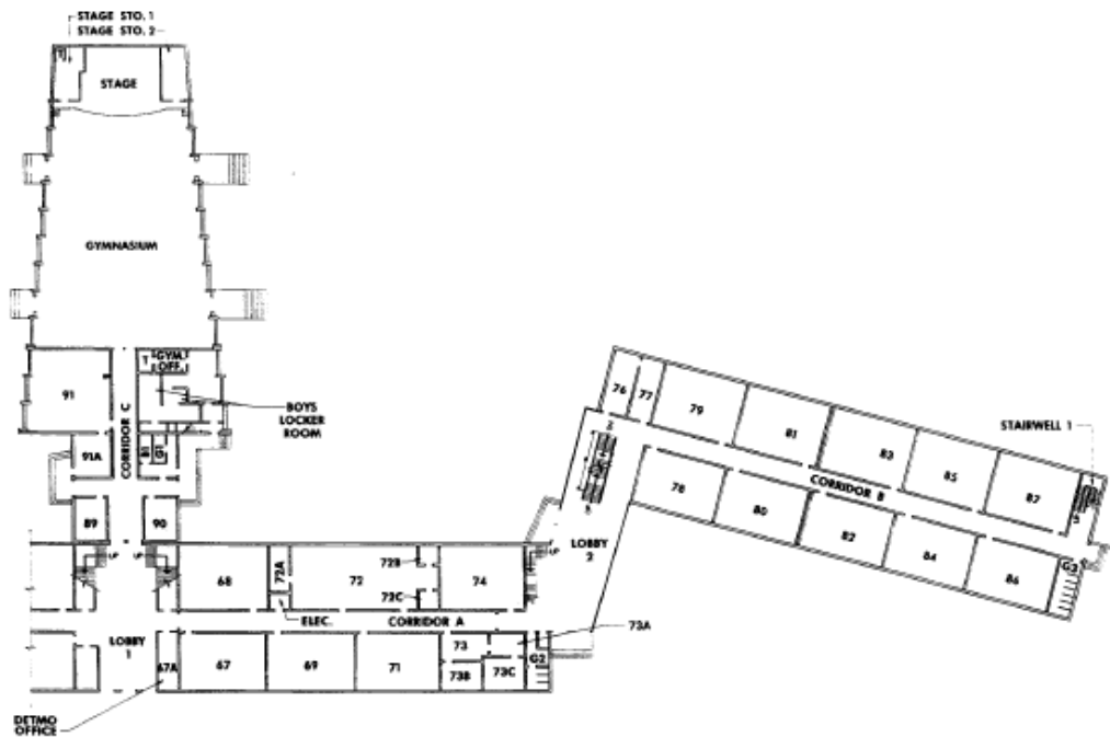
Figure 24. Middle school floor plan, Building 7778, first floor.
