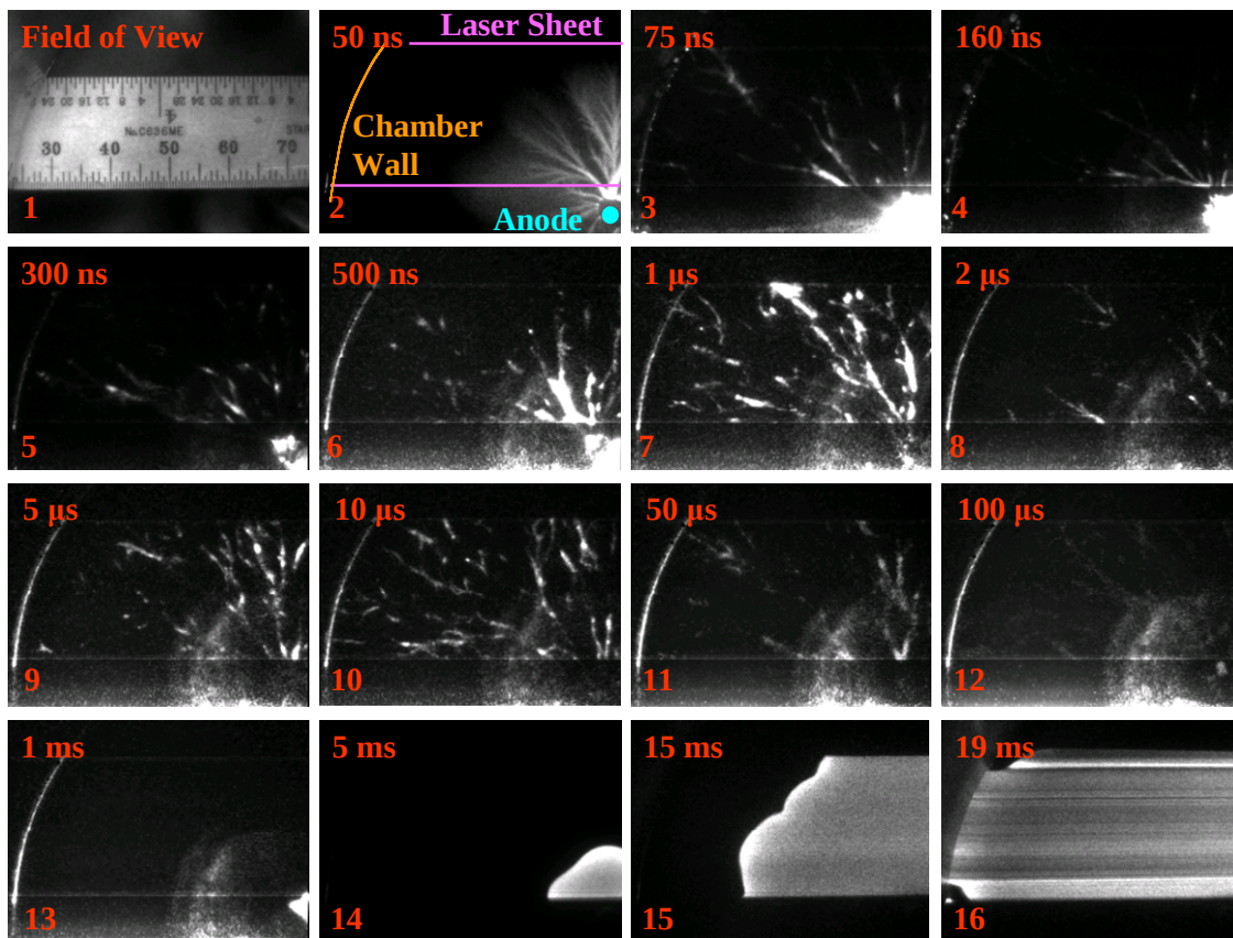
Figure 3. OH-PLIF images during CH 4 /air combustion, \phi = 1 . Intensity scaling was adjusted for maximum viewability.
