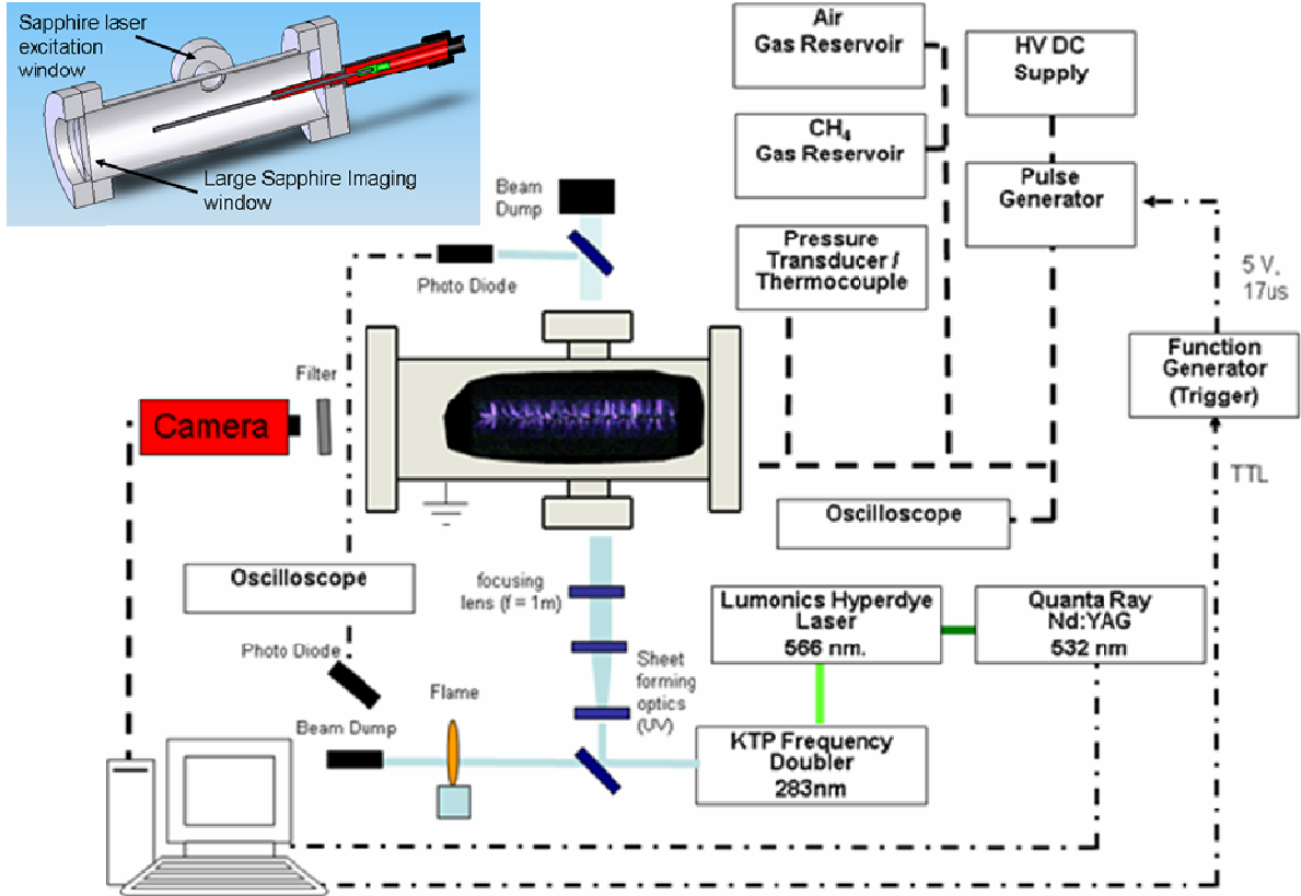
Figure 1. Schematic of the OH-PLIF experiment.
