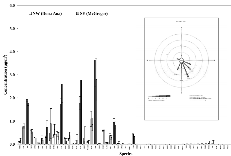
Figure 4.8. Differences in \text{PM}_{10} observed during easterly winds for the NW Dona Aña and SE McGregor monitoring sites, 17-06-01, showing a net downwind increase.
