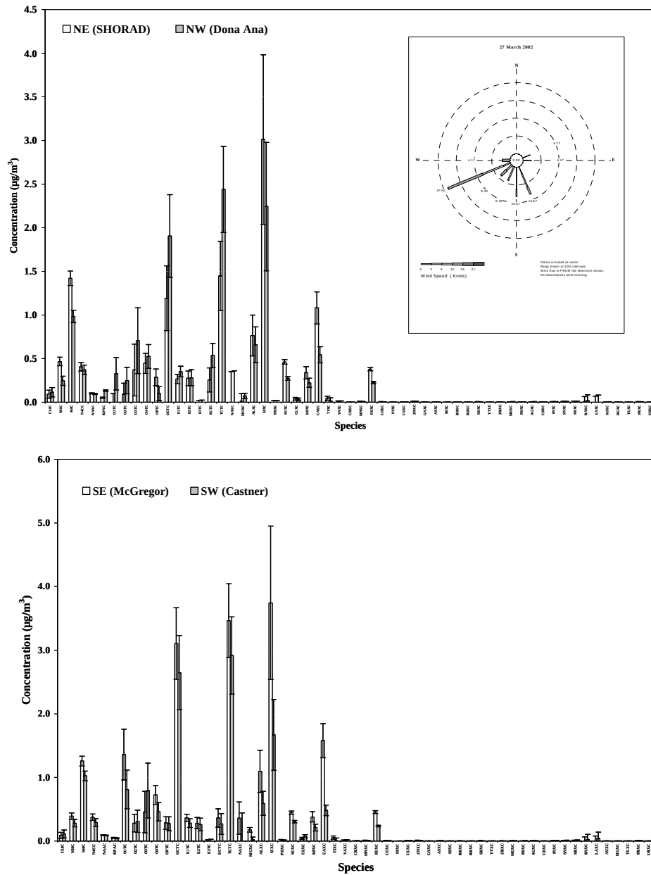
Figure 4.5. Differences in PM 10 observed during westerly winds for the north (top) and south monitoring sites, 27-03-02.
