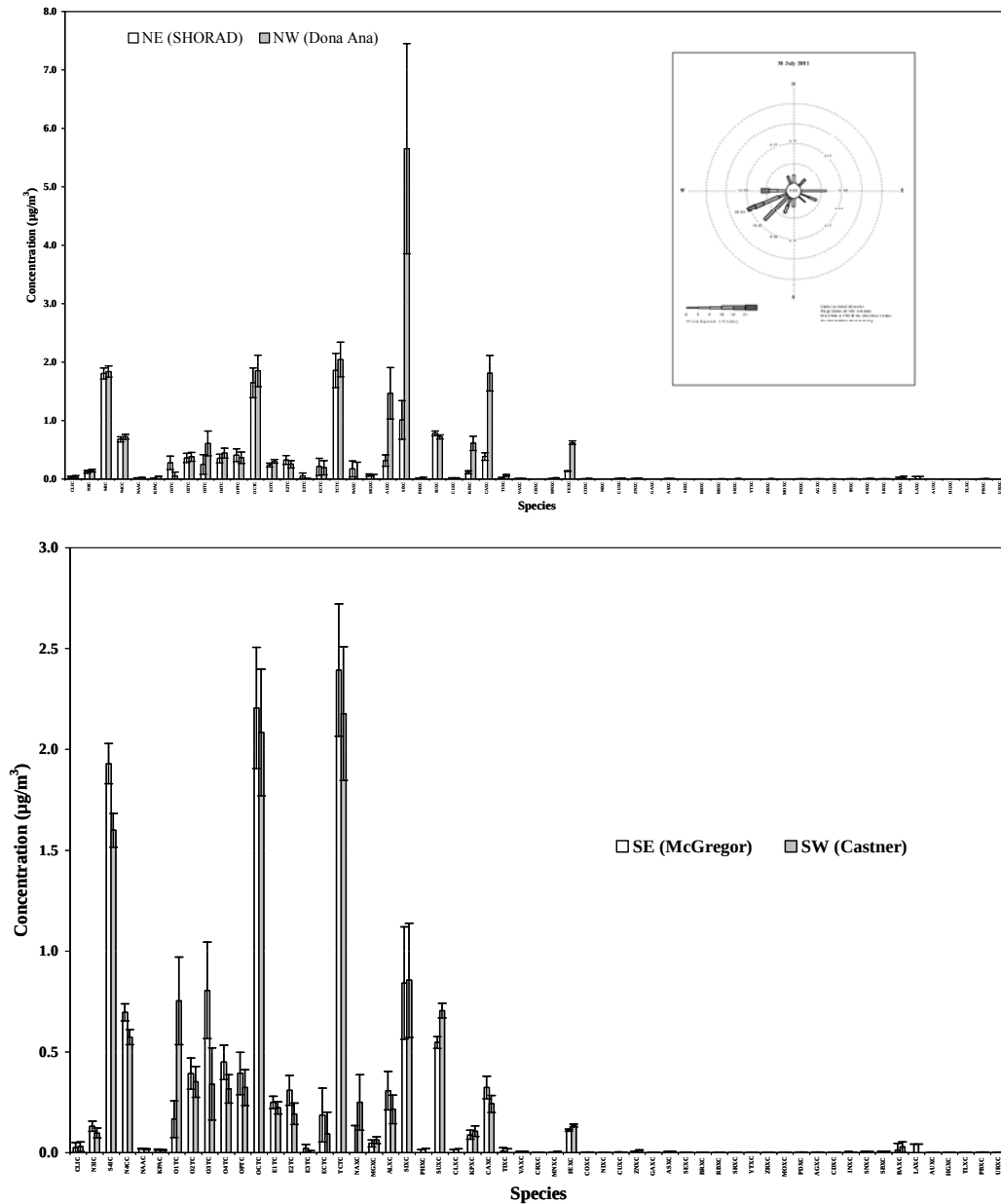
Figure 4.7. Example of the case where a net loss of PM 10 is observed on the downwind sampling location during predominantly westerly winds for the NW Dona Aña and NE SHORAD monitoring sites, 30-07-01.
