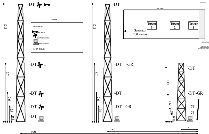
Figure 4.35. Experimental setup for the fugitive dust study at Ft. Bliss near El Paso, TX.
