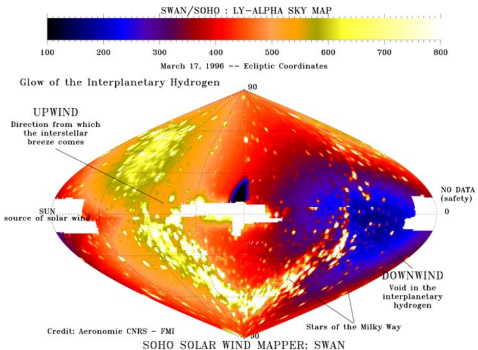
Figure 1 SWAN Lyman- \alpha whole sky map in ecliptic coordinates. The area around the Sun and the anti-solar direction were not covered for safety reasons. The color represents intensity, in counts per second per pixel (one square degree), corresponding to increments of 1.3 Rayleigh. A number of UV hot stars can be identified, tracing the galactic plane. The rest of the ubiquitous emission is due to solar UV Lyman- \alpha photons, backscattered by hydrogen atoms in the solar system. These H atoms are coming from interstellar space, and are approaching the Sun within about 2 AU, in the direction of the incoming flow (ecliptic coordinates; longitude 254^\circ , latitude 7^\circ ). A maximum of Lyman- \alpha intensity surrounds this upwind direction. In the opposite direction, the emission is weaker by a factor of 3.5, because most atoms have been destroyed by charge exchange with solar wind protons, creating a cavity void of neutral hydrogen atoms in the downwind direction. A detailed comparison of such Lyman- \alpha maps allows the solar wind mass flux to be determined at all ecliptic latitudes (Bertaux et al. , 1997).
