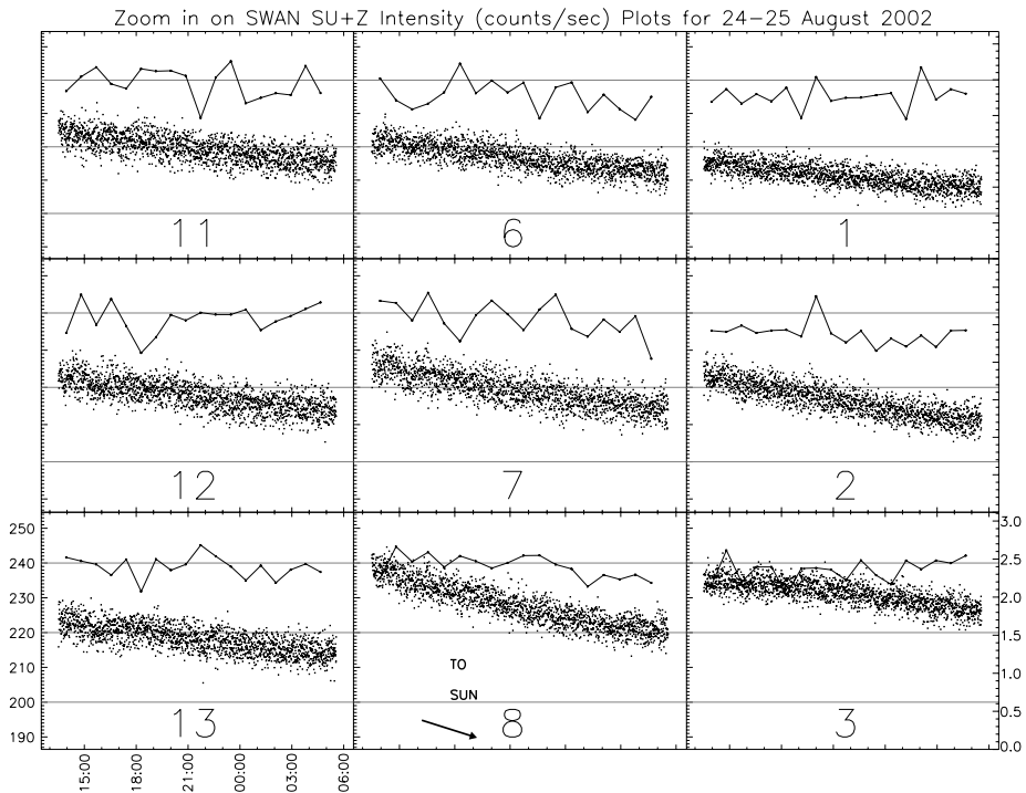
Figure 5 Zoom in on pixels of interest in Figure 3 of the intensity (counts/s) vs. time plots for SWAN observing period 24–25 August 2002. The running standard deviation, calculated every 100 points, is plotted against the opposite y-axis and shown as a solid line.
