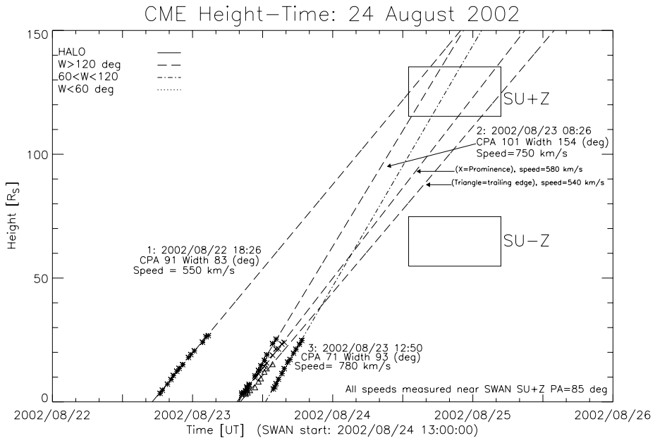
Figure 6 CME extrapolated height-time plot from LASCO data for SWAN observation period 24 August 2002. The three CMEs are denoted by the dashed lines with asterisks. The two other dashed lines are the height-time extrapolation for the prominence and trailing edge of the second CME on 2002/08/23 08:26 UT, denoted by the crosses and triangles respectively. The two boxes represent the radial width of the SU+Z and SU-Z sensors in height and observations duration in time.
