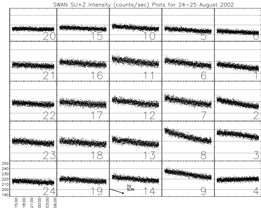
Figure 3 Intensity (counts/s) vs. time plots of 25 SU+Z sensor pixels for SWAN observing period on 24–25 August 2002. SWAN SU+Z was located at 122 R_S and 85^\circ . These plots are positioned to correspond to SU+Z pixel locations and the arrow shows the line towards the Sun given the sensor configuration shown in Figure 2.
