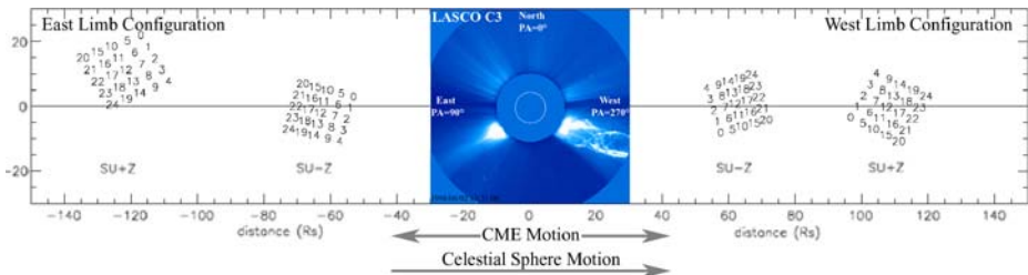
Figure 2 LASCO C3 (3.7 to 30 R_S ) and SWAN SU-Z and SU+Z (20 R_S \times 20 R_S ) sensor configurations for the east and west limbs during the observing campaign. The location of each SWAN sensor pixel is denoted by the pixel number. The directions of celestial sphere and CME motion are indicated.
