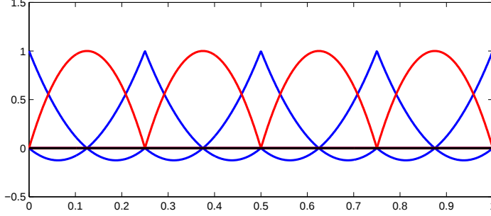
Fig. 11. Basis functions for the quadratic p -method.
