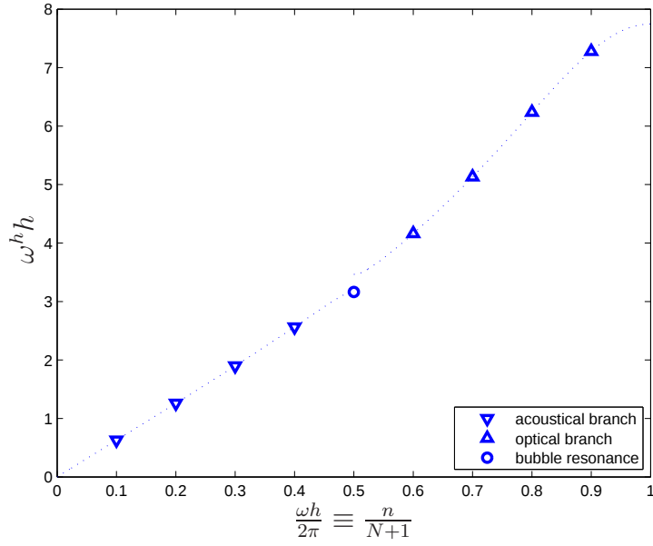
Fig. 15. Analytically-computed (discrete) natural frequencies for quadratic p -method ( N = 9 ).
