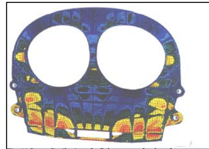
Fig. 2 Stress distribution of a fighter centre fuselage frame
