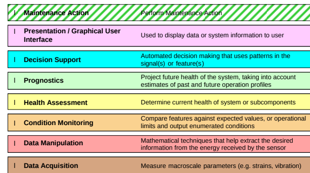
Figure 4. Functional Concept
