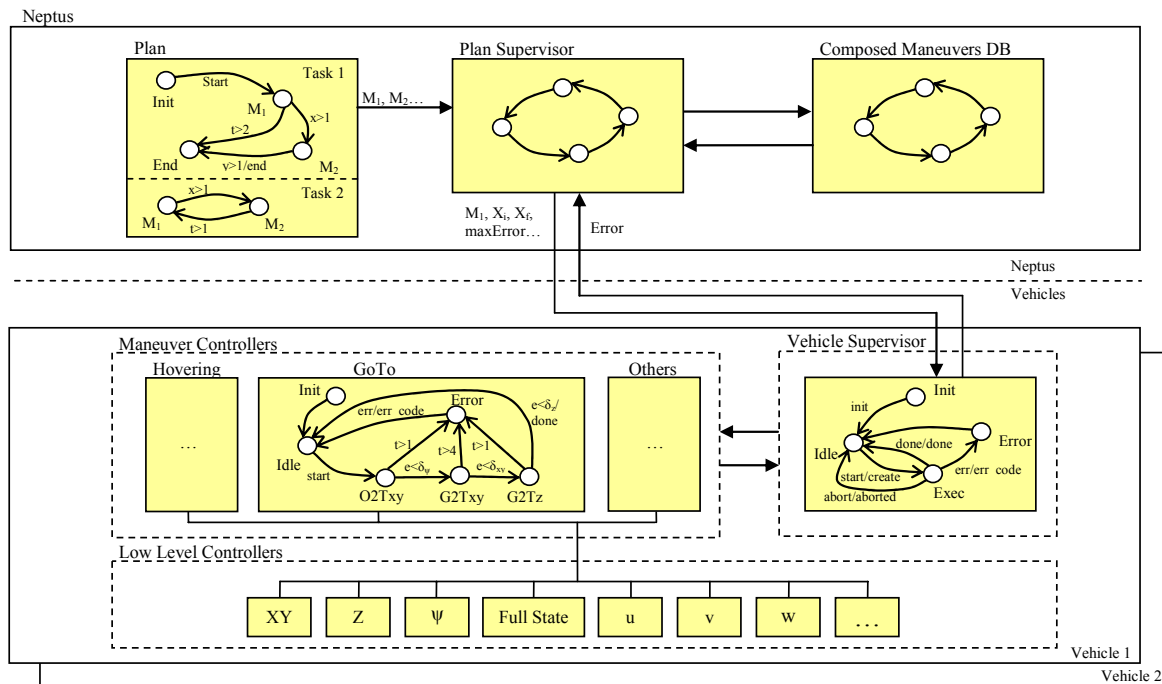
Fig. 1. Control Architecture
