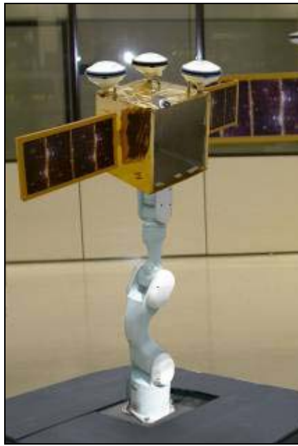
Fig. 6: S/C mock-up mounted at the top of the robotic arm
