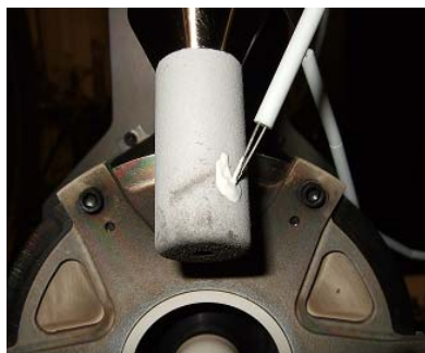
Figure 29. Thermocouple 2 Location
