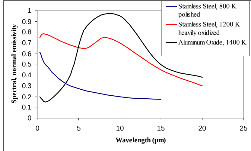
Figure 7. Wavelength Dependence of Emissivity 14
