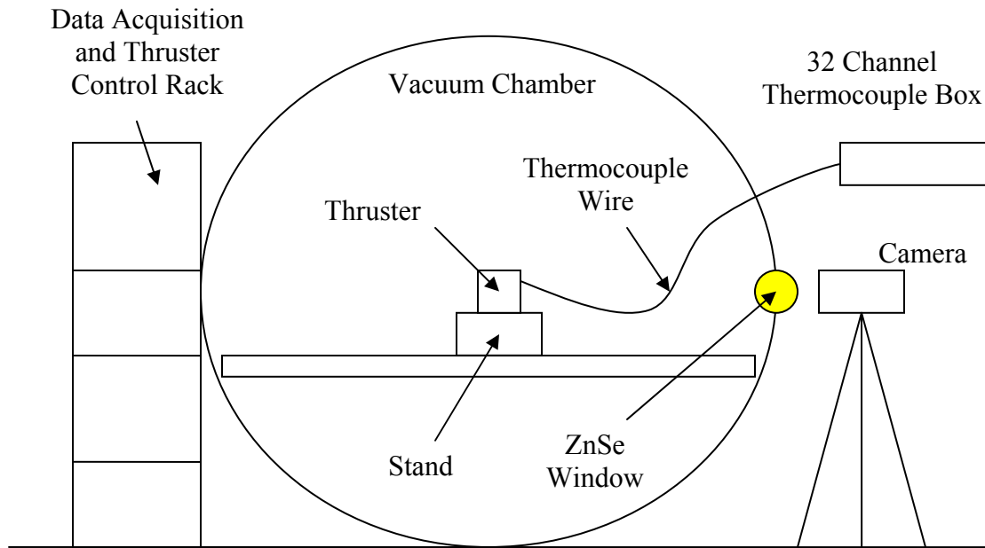
Figure 27. Experimental Setup
