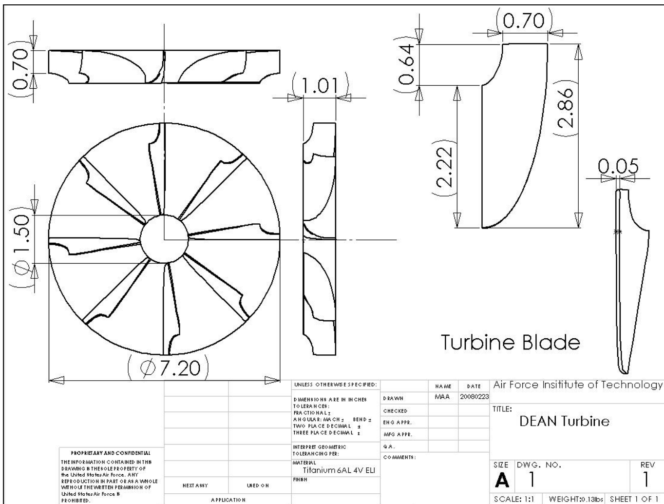
Figure 74 DEAN Turbine
