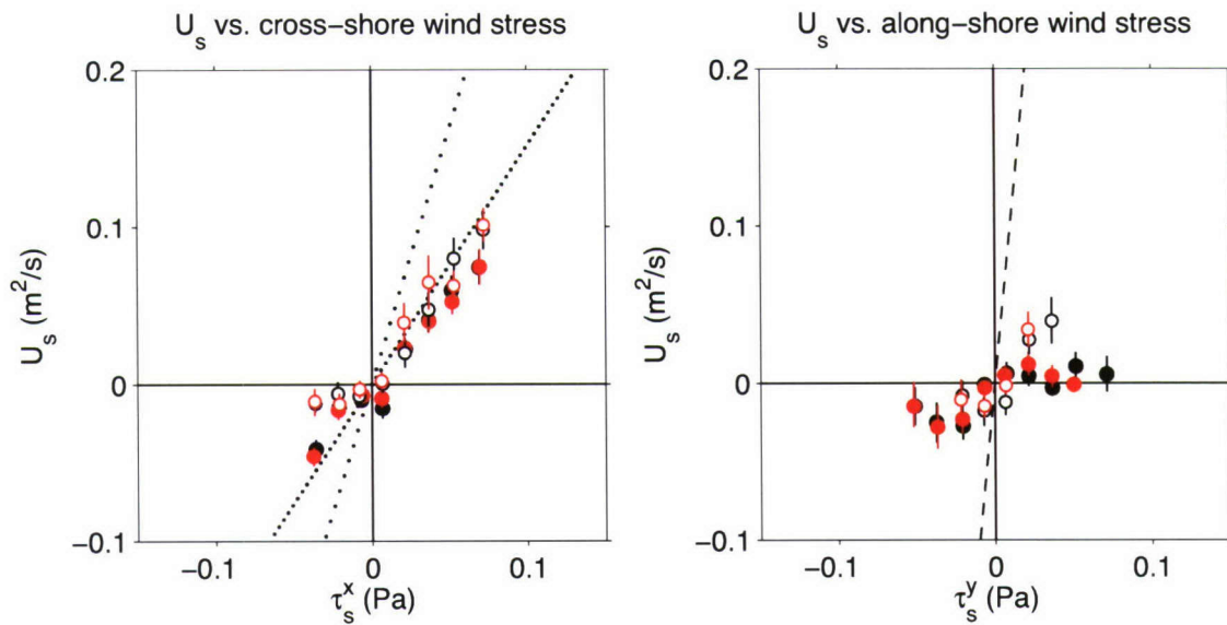
Figure A-6: Same as Figure 2-9, but with ASIT wind stress (red) and adjusted wind stress from shore masts (black), using only times when both wind stress time series are available.
