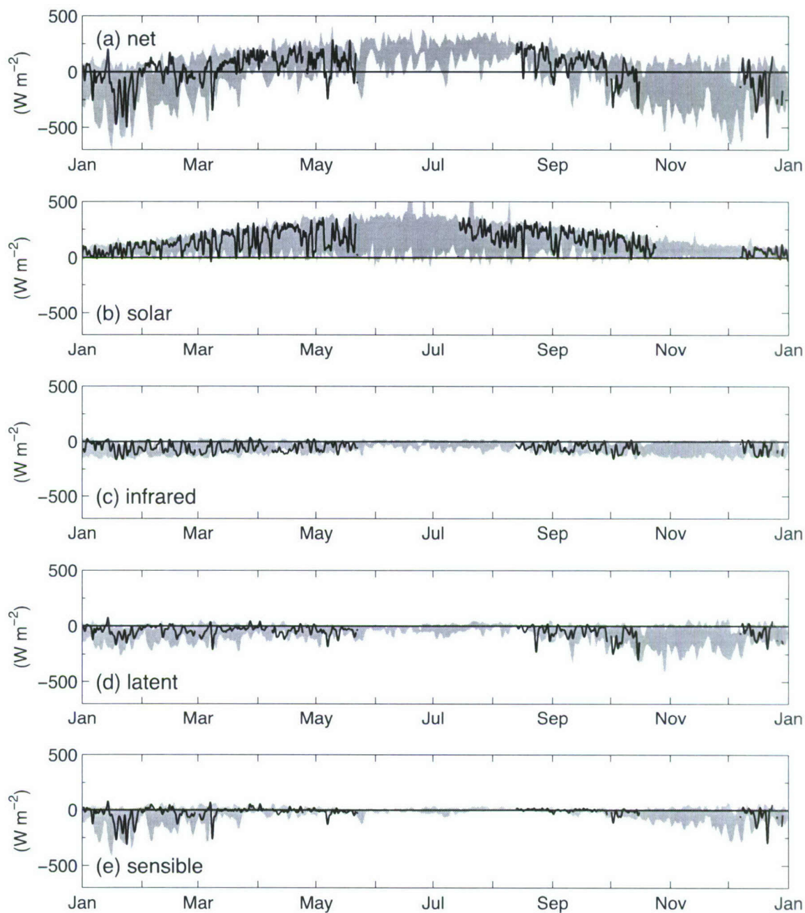
Figure 4-6: 33-hr low-pass filtered net surface heat flux Q_s and its components at the Node. Positive heat flux indicates ocean is warming. Black line: CBLAST 2003 (summer) and SWWIM I (winter/spring). Grey shading: envelope of other measurements at MVCO (2001-2007).
