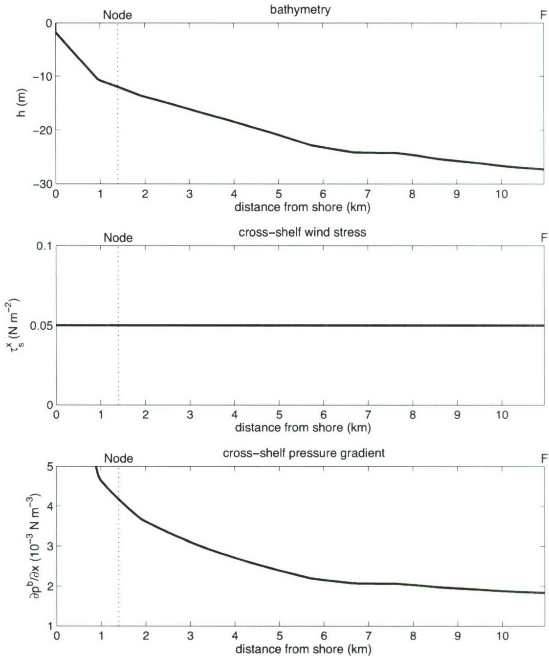
Figure 3-17: Cross-shelf structure of a cross-shelf pressure gradient due to cross-shelf wind stress alone. Top panel: the bathymetry h(x) at MVCO along a cross-shelf section from shore to mooring F, in the F coordinate system \hat{y} direction from CBLAST 2003. Middle panel: the cross-shelf wind stress (assumed constant and offshore, with \tau_s^x = 0.05 \text{ N m}^{-2} ). Bottom panel: the cross-shelf pressure gradient if the cross-shelf momentum balance is exactly a wind-driven coastal set-down balance, with \partial p^b / \partial x = \tau_s^x / h and \tau_s^x as in the middle panel.
