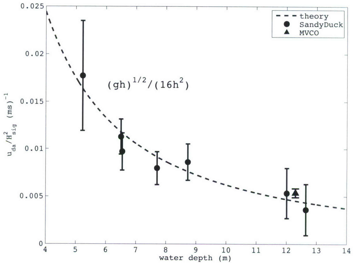
Figure E-4: Linear regression slope of u_{da} versus H_{sig}^2 as a function of water depth for the seven SandyDuck sites and MVCO. Dashed line is theoretical dependence of u_w/H_{sig}^2 on water depth based on (E.3). The error bars indicate the 95% confidence intervals on the regression slope estimates.
