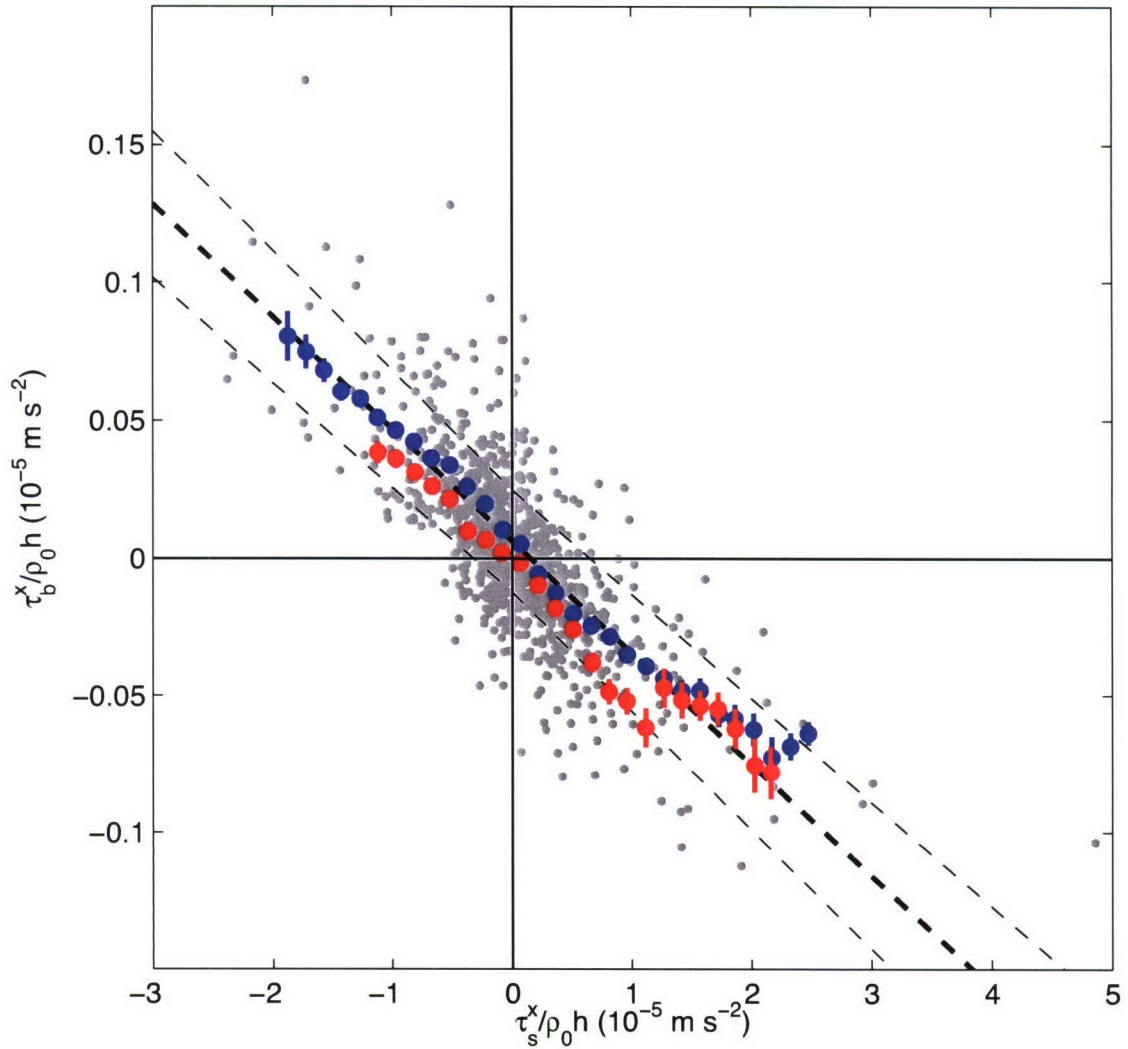
Figure 3-20: Bottom stress versus wind stress term in the cross-shelf momentum budget. Blue (red) circles are bin-averaged winter (summer) values. Grey dots are subtidal data plotted every 33 hr, which are the points used to estimate the regression slope and intercept and correlation coefficient, but are a subset of the points that go into the bin averages. Thick dashed line is a best-fit line for winter with 95% confidence limits shown by the thin dashed lines, and has slope -0.04 \pm 0.02 and intercept (-0.006 \pm 0.003) \times 10^{-5} \text{ m s}^{-2} . The two terms are significantly correlated at the 95% confidence level in both seasons, with r = -0.75 ( |r_{95\%}| = 0.08 ) in winter and r = -0.70 ( |r_{95\%}| = 0.09 ) in summer.
