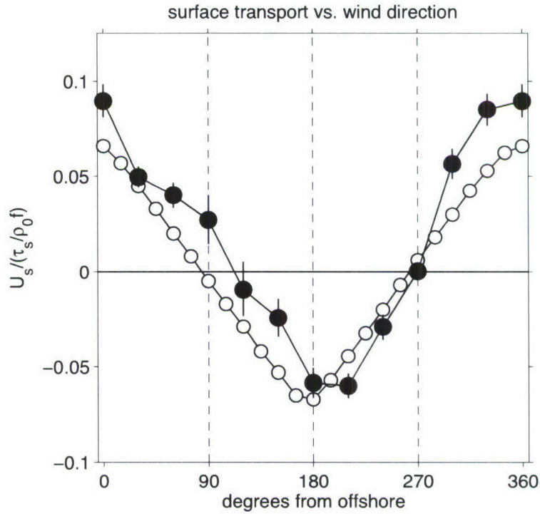
Figure 2-11: Normalized cross-shelf transport in the surface layer, U_s / (|\tau_s| / \rho_0 f) (positive offshore), as a function of wind direction. Open circles: numerical model results for |\tau_s| = 0.1 Pa and h = 5 m (taken from Tilburg, 2003, Figure 16). Solid symbols: MVCO observations for h = 12 m and 0.075 < |\tau_s| < 0.15 Pa. The cross-shelf velocity profiles were bin averaged by wind direction, then U_s was calculated, then normalized by the bin-averaged |\tau_s| / \rho_0 f . These data are restricted to times when waves are small, so there are fewer events for the onshore wind stress angles (near 180^\circ ) than for the offshore. In both the model and the observations, the largest surface layer transport is for cross-shelf, not along-shelf, winds.
