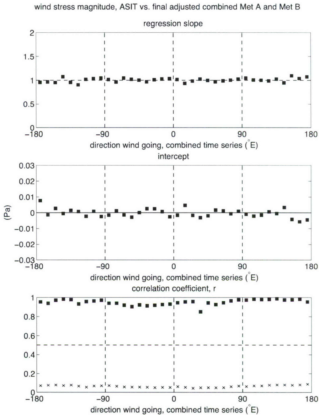
Figure A-5: Same as Figure A-1, but for wind stress magnitude of the final combined time series of wind stress from adjusted Met A and Met B.
