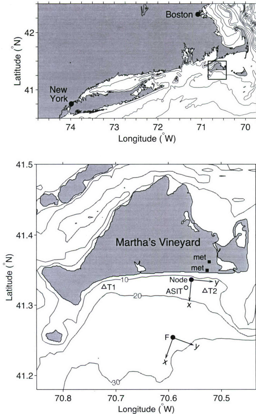
Figure 4-3: Top panel: location of detailed map of study area (square outline). Iso-baths are shown in increments of 20 m ( i.e. , the 20-m, 40-m, 60-m... isobaths). Bottom panel: detailed map of study area, with Node and F principal axis coordinate systems from CBLAST 2003 (Appendix E). Iso-baths are labeled in meters. Solid dots: moorings Node and F, deployed during CBLAST 2003 and SWWIM I. Triangles: moorings T1 and T2, deployed during CBLAST 2003 only. Circle: MVCO air-sea interaction tower (ASIT). Squares: MVCO meteorological masts.
