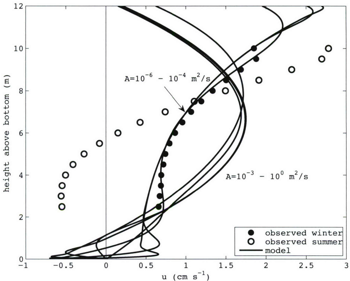
Figure E-9: Average cross-shelf velocity profiles from the model described in Section E.4.1 for various constant eddy viscosities A (lines) and observed average profiles from MVCO during winter (October - March) and summer (April - September) for 1 < H_{sig} < 2 and |\tau^s| < 0.03 \text{ N m}^{-2} . Model profiles were computed using the average significant wave height (1.3 m) and wave period (6.4 s) of the observed winter profiles (summer values are essentially the same). Standard errors of the means are 0.3 \text{ cm s}^{-1} for the winter profile and 0.5 \text{ cm s}^{-1} for the summer profile.
