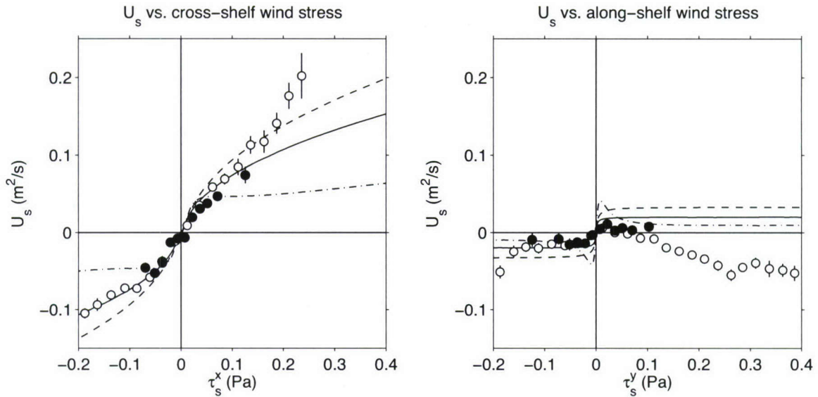
Figure 2-10: Cross-shelf transport in the upper water column, U_s (positive offshore), as a function of (left) cross-shelf or (right) along-shelf wind stress, during winter. Solid symbols: U_s during small waves and weak |\tau_s^y| (left) or |\tau_s^x| (right). Open symbols: U'_s , which is U_s during any wave conditions and weak |\tau_s^y| (left) or |\tau_s^x| (right), but with the predicted wave-driven velocity profile u_H(z, t) = -u_{st}(z, t) (Hasselmann, 1970) subtracted from u(z, t) before calculating U_s . Error bars are \pm one standard error of the mean. Lines indicate the U_s predicted by a simple numerical model with constant density and the MYApprox, cubic, or bilinear cutoff eddy viscosity profile (dashed, solid, or dash-dot line, respectively, forced by (left) cross-shelf or (right) along-shelf wind stress (Lentz, 1995).
