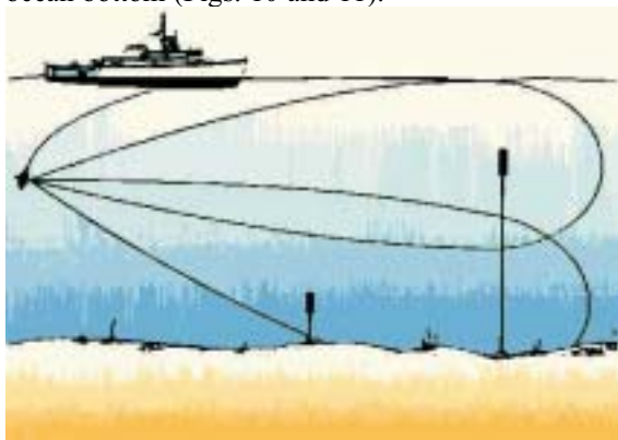
Fig. 9. AN/SQQ-32 Concept.
