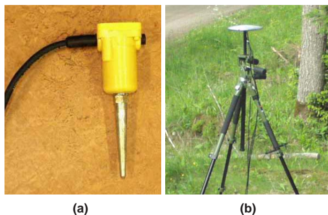
Figure 3: Sensors used in the IAM project. In (a) the geophone, put into the ground in arrays of three. In (b) an acoustically well-designed microphone array mounted on an ordinary microphone stand. The disc contains three microphone elements.
