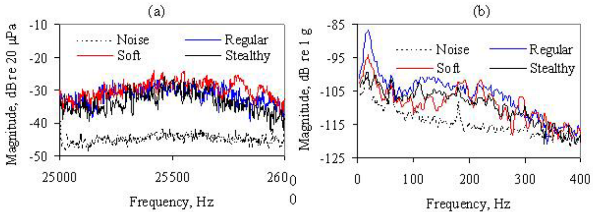
Figure 3. Average Fourier spectra of ten regular, soft, and stealthy footsteps on the ground. (a) is the sound pressure at 5-7 m from a walker and (b) is the acceleration at 1 m from a walker. The sampling rate was 64 kHz and the FFT size was 32,768.
