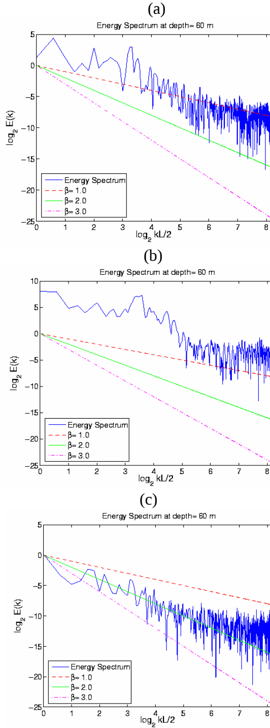
Figure 10. Power spectra of temperature at 60 m deep on (a) 1000-1500 GMT July 29 (IW-turbulence), (b) 0700-1200 GMT July 30 (IS-turbulence), and (c) 0000-0500 GMT August 1 (turbulence-dominated), 2005.
