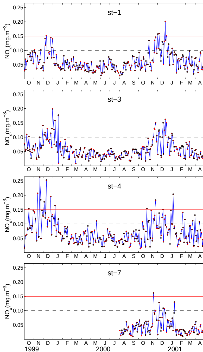
Figure 4. Daily mean NO x concentrations (mg m -3 ) at St-1, St-3, St-4 and St-7 representing four districts. Horizontal dashed line is daily mean second-level criterion, while horizontal solid line is daily mean third-level criterion.
