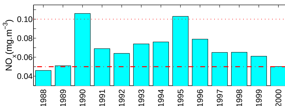
Figure 3. Annual mean NO x concentration ( \text{mg m}^{-3} ) measured at the local CEPA station (103.631°E, 36.103°N), which is marked as the solid circle in Fig. 1b. The second-level criterion is represented by the horizontal dash-dotted line and the third-level criterion is represented by the horizontal dotted line.
