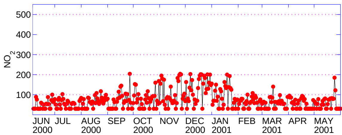
Figure 5. Daily mean API of NO 2 at station-E.
