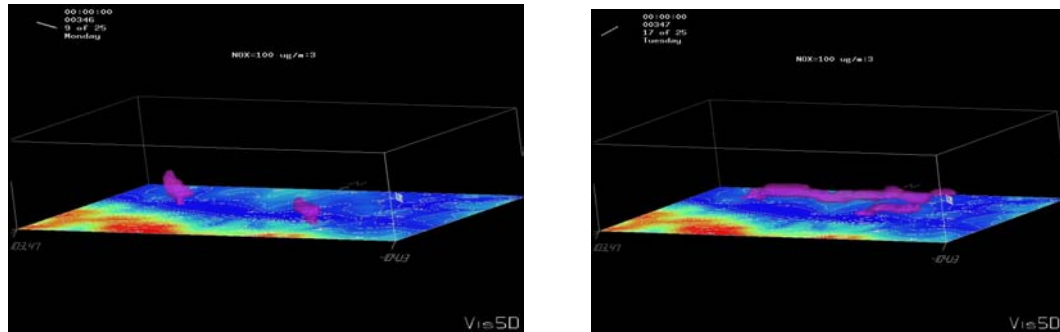
Figure 9. Model simulated NOx plume (concentration > 0.1 mg/m 3 ) spreading and enhancing from (a) 0700 BT, Dec 11 to (b) 0700 BT, Dec 12, 2000.
