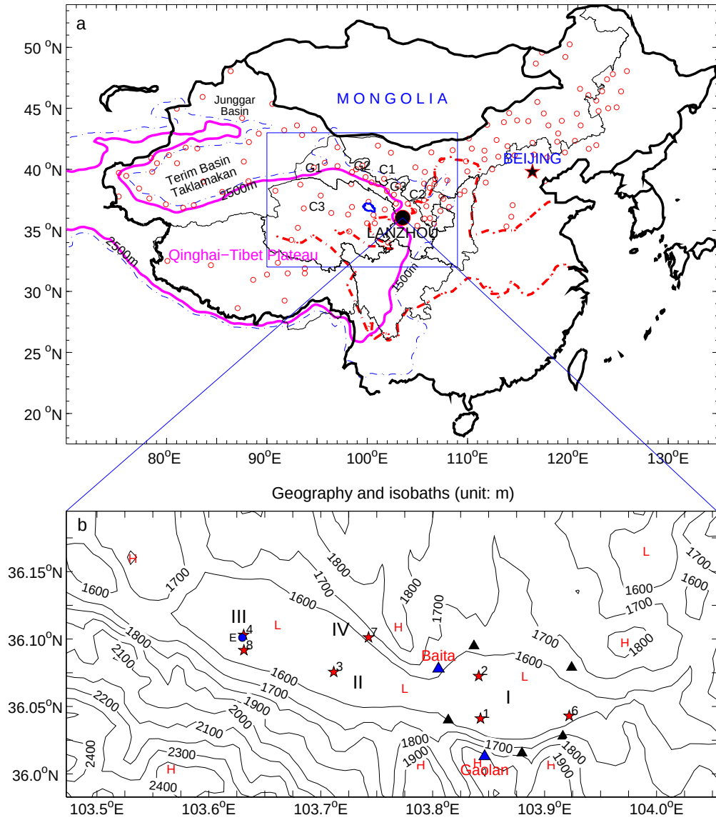
Figure 1: Lanzhou: (a) geography and (b) topography.
