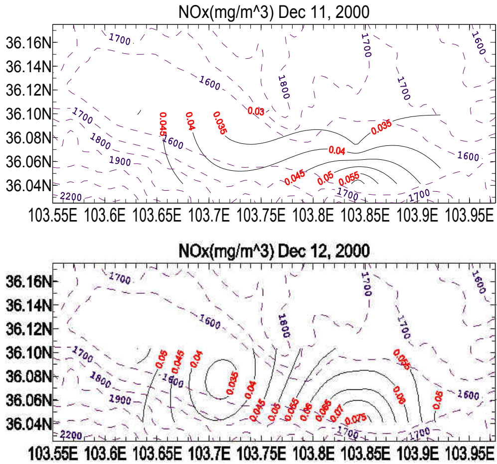
Figure 10. Observed NO x concentration on (a) December 11, and (b) December 12, 2000.
