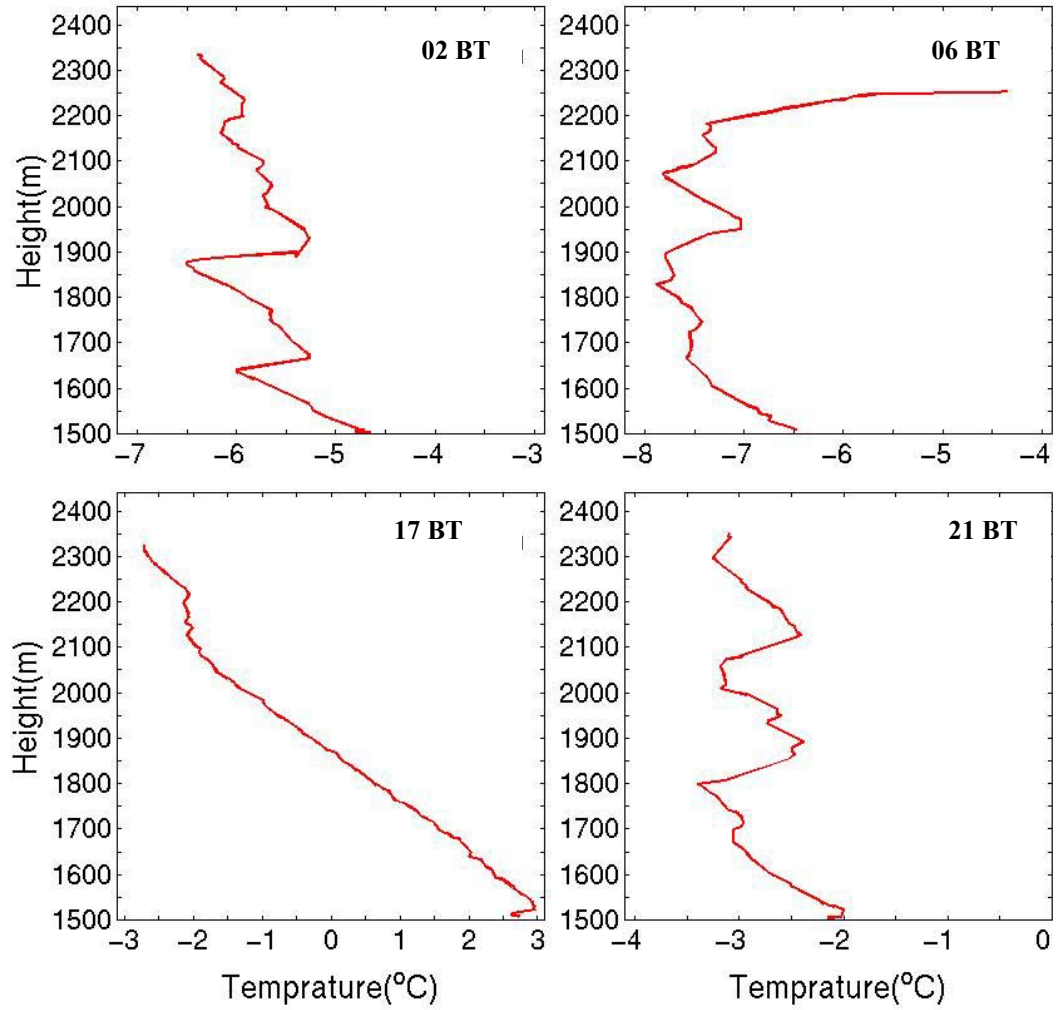
Figure 7. Model simulated and horizontally averaged temperature profiles over the grid-5 region (i.e., Lanzhou) on December 11, 2000: (a) 0200 BT, (b) 0600 BT, (c) 1700 BT (three hours after the local noon time), and (d) 2100 BT.
