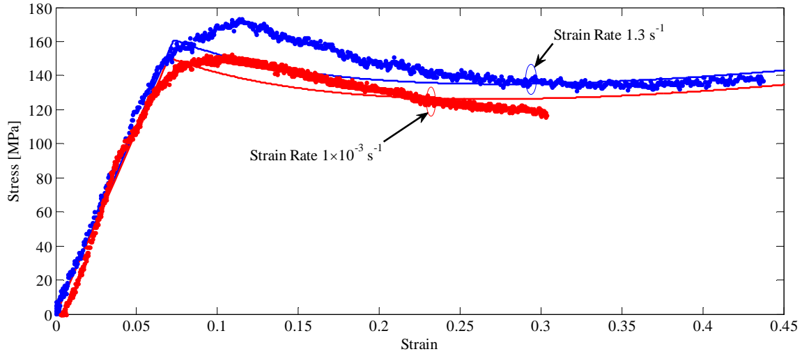
Figure 2. Experimental data ( \bullet ) and 1D Mulliken-Boyce model output ( - ) using best estimates (Table 1).
