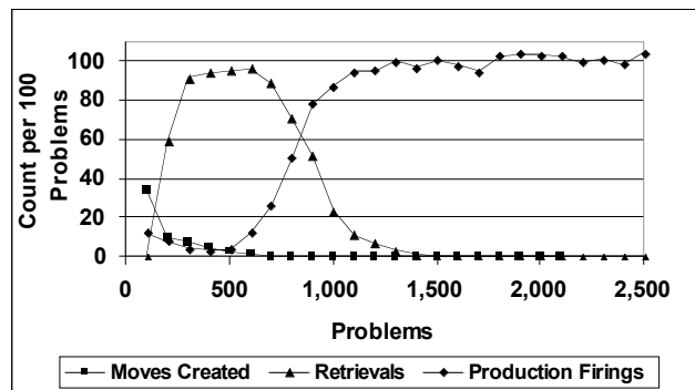
Figure 4. ACT-R Stages of learning
