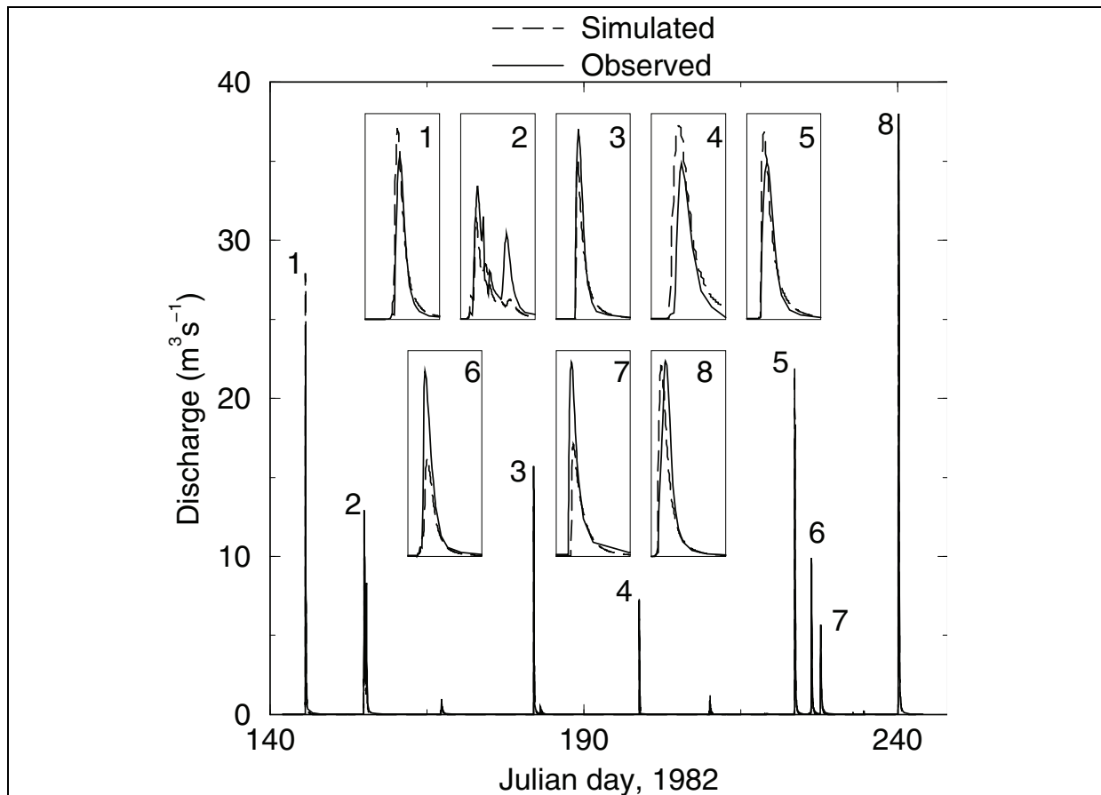
Figure 2. Observed and simulated discharges for the calibration period at GCEW outlet gage.
