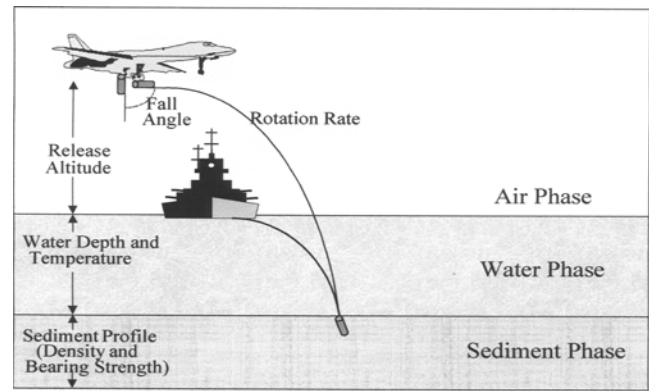
Fig. 1. The trajectory of a cylindrical mine as it falls through three phases: air, water, and sediment. Labels are parameters used by the model to calculate the velocity, attitude, and burial depth of the mine.
