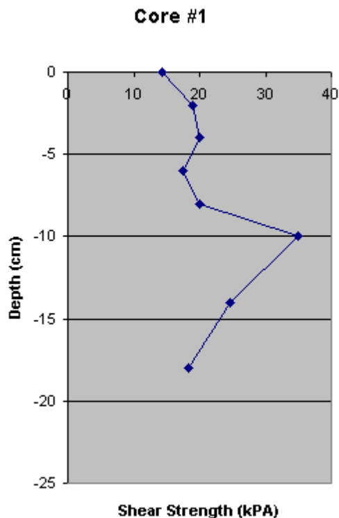
Fig. 5 Sediment shear strength profile at the gravity core #1.
