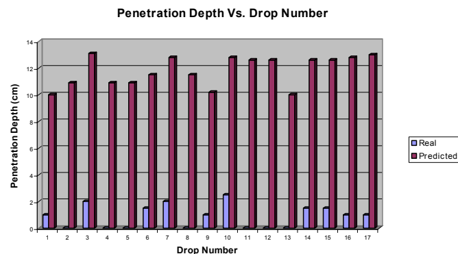
Fig. 9. Comparison between measured and modeled mine burial depths. Here maroon and blue bars indicated modeled and measured values.
