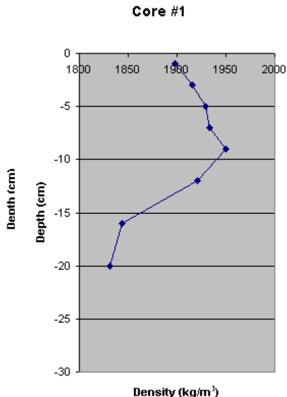
Fig. 4 Sediment density profile at the gravity core #1.
