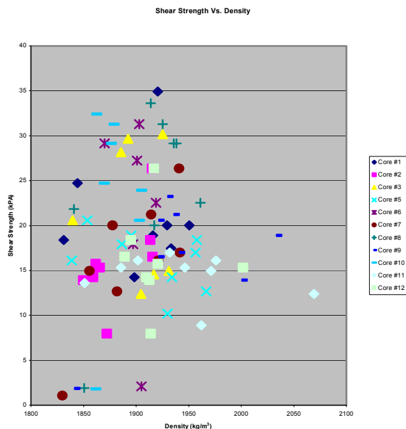
Fig. 6. Shear strength versus density near MISO at Del Monte beach of the Monterey Bay.
