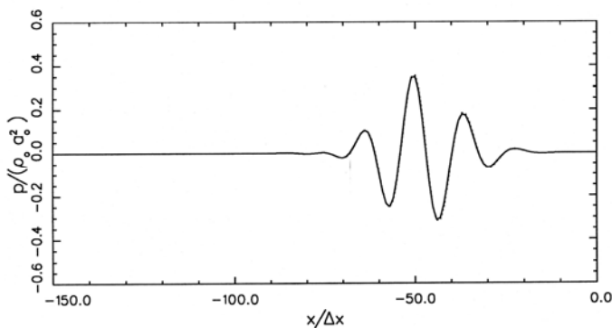
Figure 9.11 Pressure waveform of the reflected acoustic pulse at t = 140.1 .
