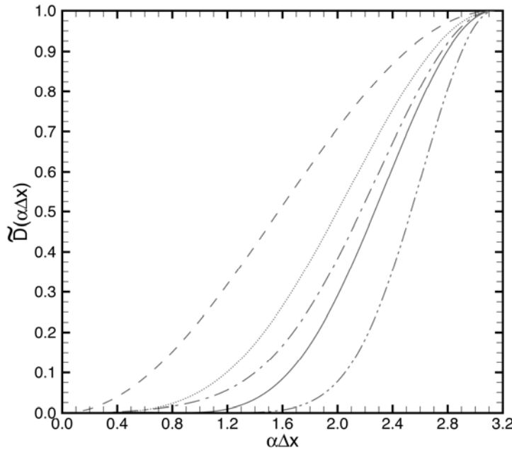
Figure 4.5. Damping functions \tilde{D}(\alpha\Delta x) . — 7-point stencil ( \sigma = 0.2\pi ), ——— 7-point stencil ( \sigma = 0.3\pi ), ..... 5-point stencil, - - - 3-point stencil, - · - · - 15-point stencil.
