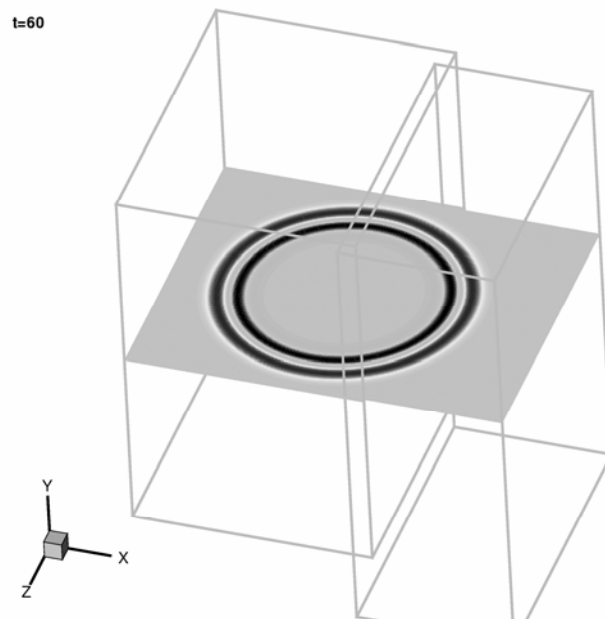
Fig.7.25. Computed pressure contours in the x-z plane at t = 60 .
