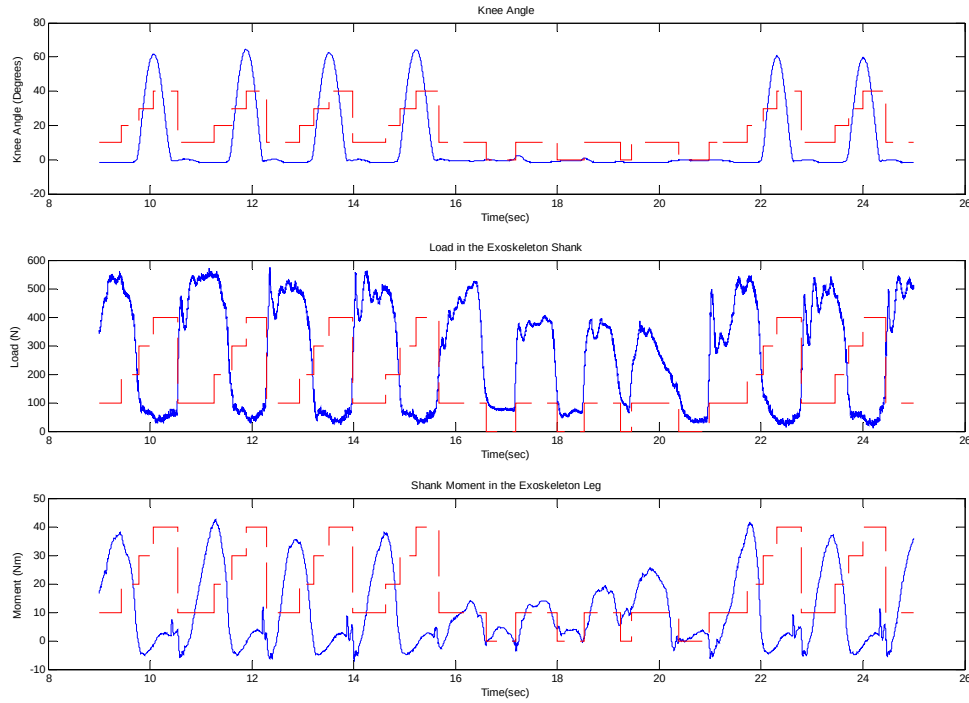
Figure 4.11 The state machine for the exoskeleton knee in operation. The data shows the person walking normally, then shuffling as they turn around and then walking some more.
