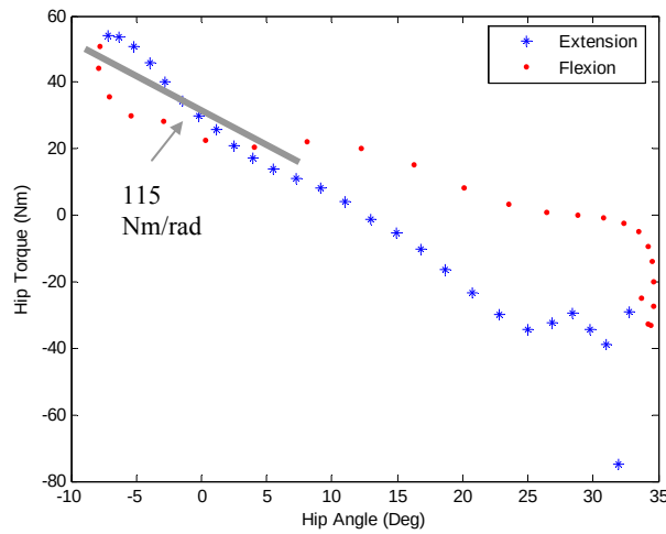
Figure 2.9 The hip angle plotted versus hip torque for a walking speed of 0.8m/s (Kirtley, 1998 (old)).
