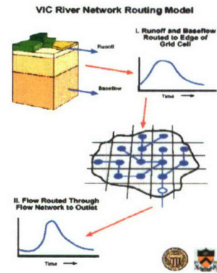
Fig. 3 University of Washington's VIC River Routing Model.
