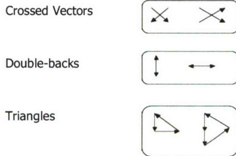
Fig. 5 Types of flow-direction errors after network adjustment
