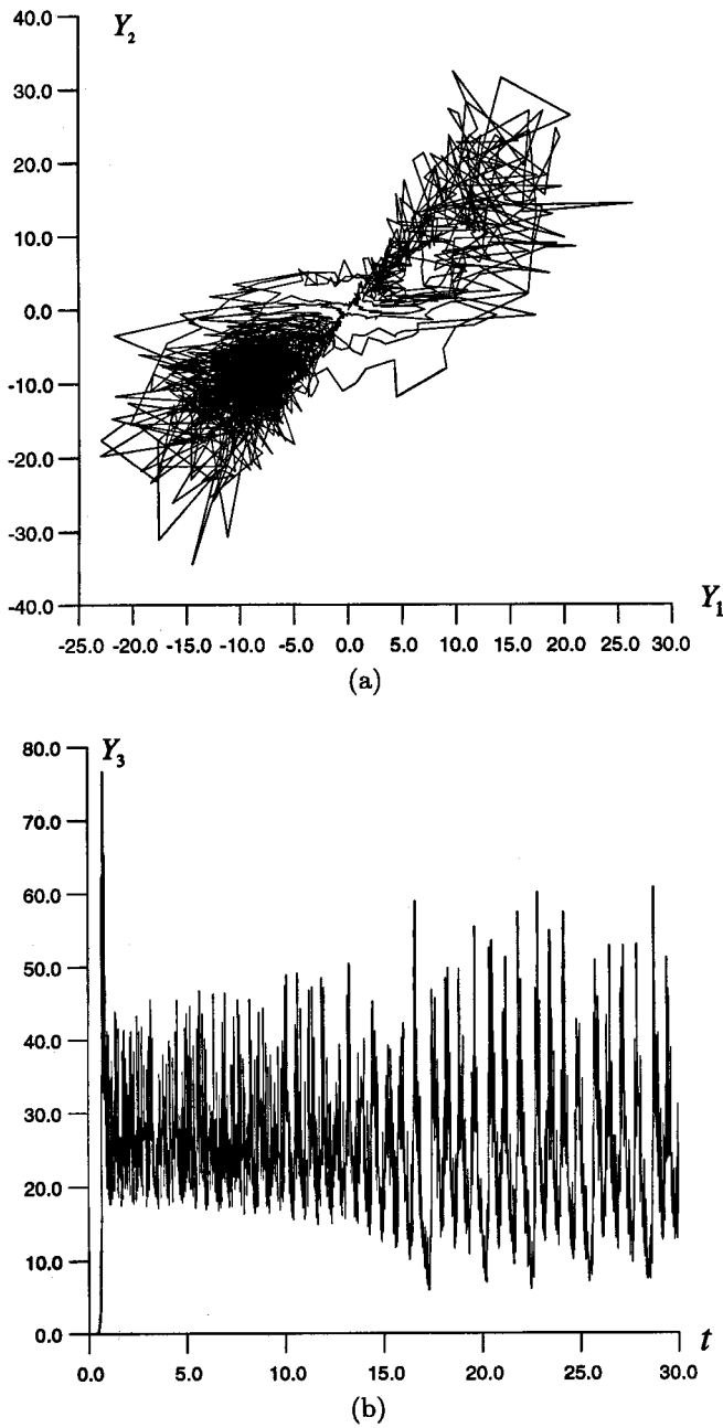
Fig. 4. Lorenz attractor distorted by white noise with \eta_1 = 0.6 : (a) noisy track in (Y_1, Y_2) phase space with no butterfly pattern, (b) time series of Y_3 .
