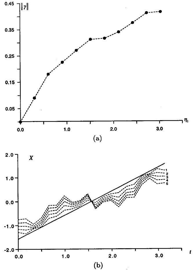
Fig. 1. Reconstruction of the one-dimensional linear process: (a) upper panel: reconstruction accuracy, and (b) lower panel: comparison between \bar{Y}(t) (solid line) and reconstructed processes X(t) (dashed curves) with 1, 2, 3, 4 and 5 corresponding to \eta_1 = 0.6, 1.2, 1.8, 2.4 , and 3.0 .
