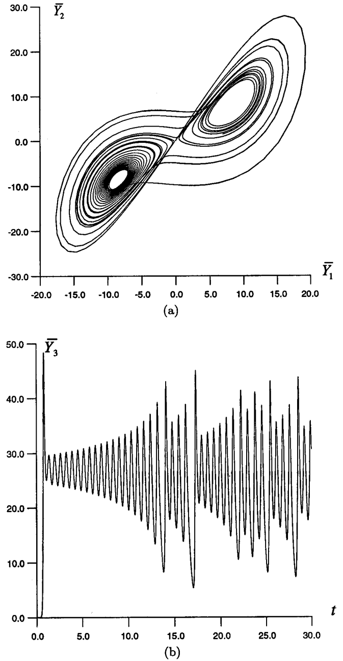
Fig. 5. Reconstructed Lorenz attractor from the "noisy data" with \eta_1 = 0.6 using the rotation method: (a) butterfly pattern of track in (\bar{Y}_1, \bar{Y}_2) phase space, (b) time series of \bar{Y}_3 .
