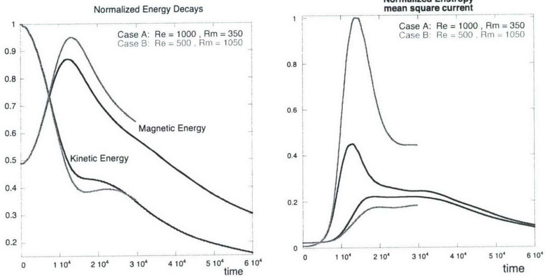
(a) normalized kinetic and magnetic energy (b) normalized kinetic and magnetic enstrophy
