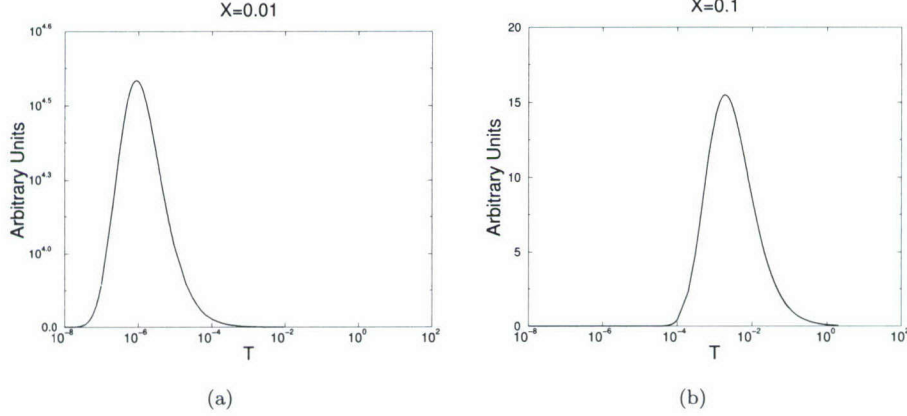
FIG. 1.2. The wavefront impulse response (1.15) at two depths for \alpha = 0.7 .
