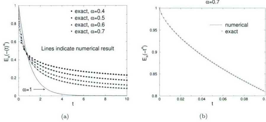
FIG. 1.10. (a) Demonstration of accuracy of scheme to compute fractional derivatives; (b) demonstration of accuracy obtained with the scheme near t = 0 .
