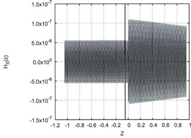
FIG. 7: Magnetic field profile of the Stokes wave. Pumping frequency 12GHz.
