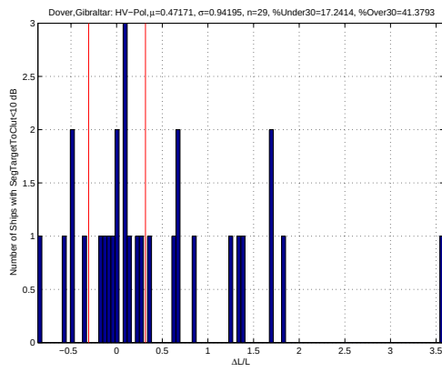
Figure 37: Histograms of \Delta L/L for ships with TCR < 10 dB showing the 30% error positions (red lines) for each linear polarization.
