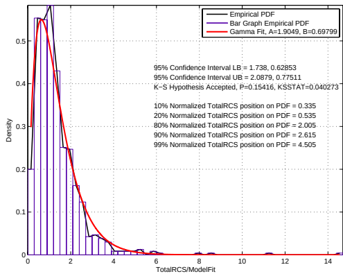
Figure 30: Combined co-polarization and cross-polarization PDF (left) and ECDF (right). The original co-polarization data set (1 st row) did not pass the K-S test; however, it does pass the K-S test (2 nd row) after removing the two largest normalized total RCS samples from the data set.
