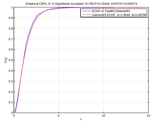
Figure 30: Combined co-polarization and cross-polarization PDF (left) and ECDF (right). The original co-polarization data set (1 st row) did not pass the K-S test; however, it does pass the K-S test (2 nd row) after removing the two largest normalized total RCS samples from the data set.
