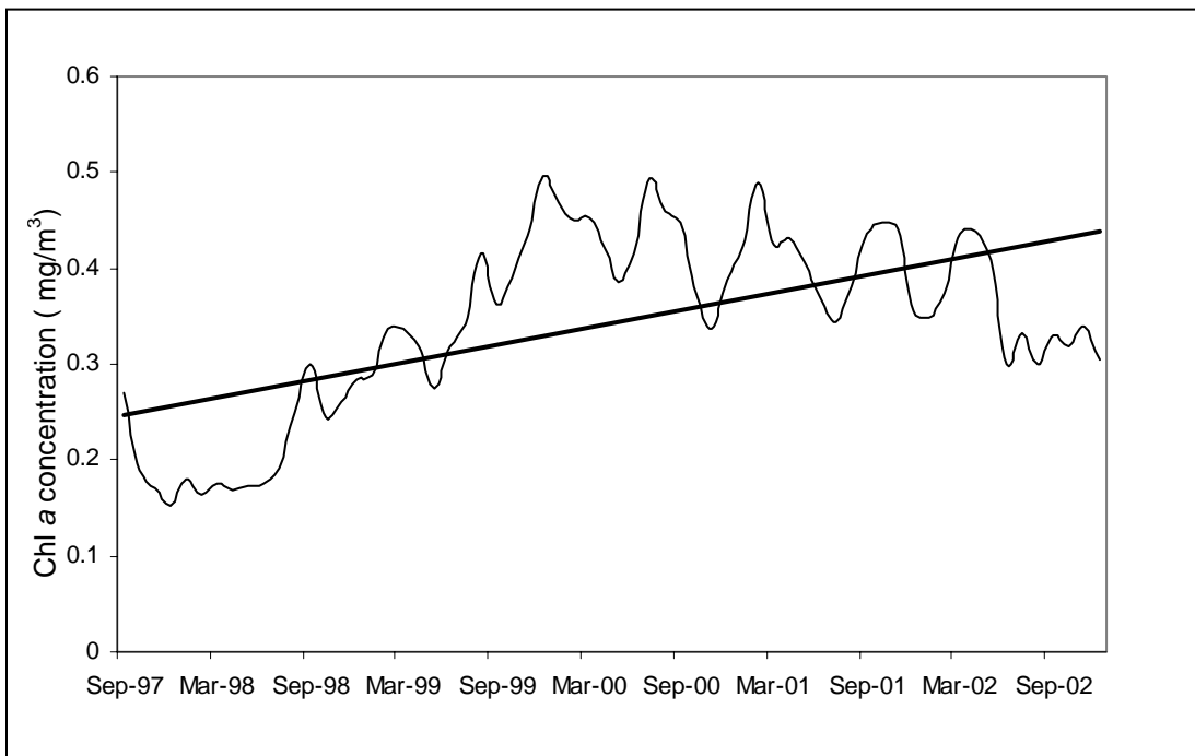
Figure 6. Time series of chlorophyll a data from SeaWIFS showing low levels during 1997-1998 and an overall increase in the broad study area from 1997-2002. Data were only available starting in September 1997.
