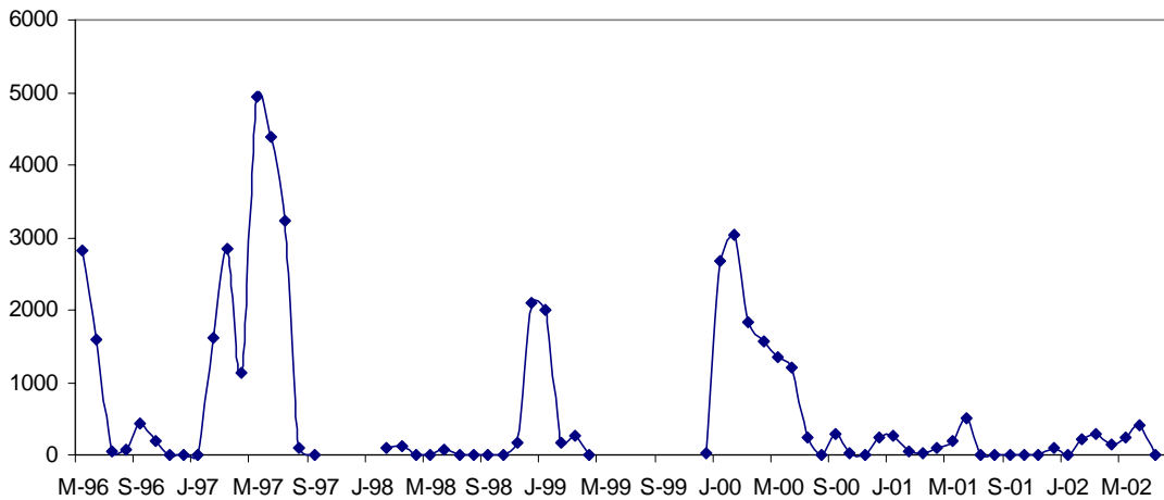
Figure 2. Number of blue whale "B" calls detected by year at 8°N 95°W from May 1996-October 2002. Data were unavailable from October 1997-February 1998 and from June 1999-December 1999.
