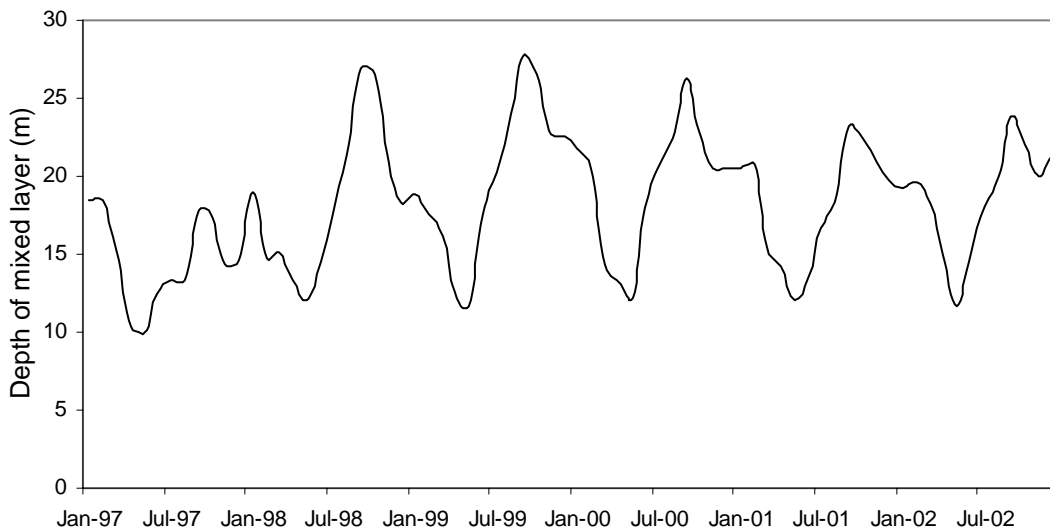
Figure 8. Mixed layer depth for the northern eastern tropical Pacific.
