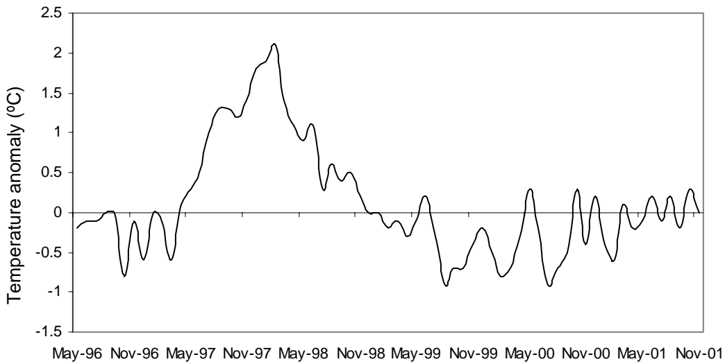
Figure 7. Sea surface temperature anomaly data (time series minus the long term mean) for the eastern tropical Pacific. Note that the El Niño year shows values well above the expected mean for almost 18 months.
