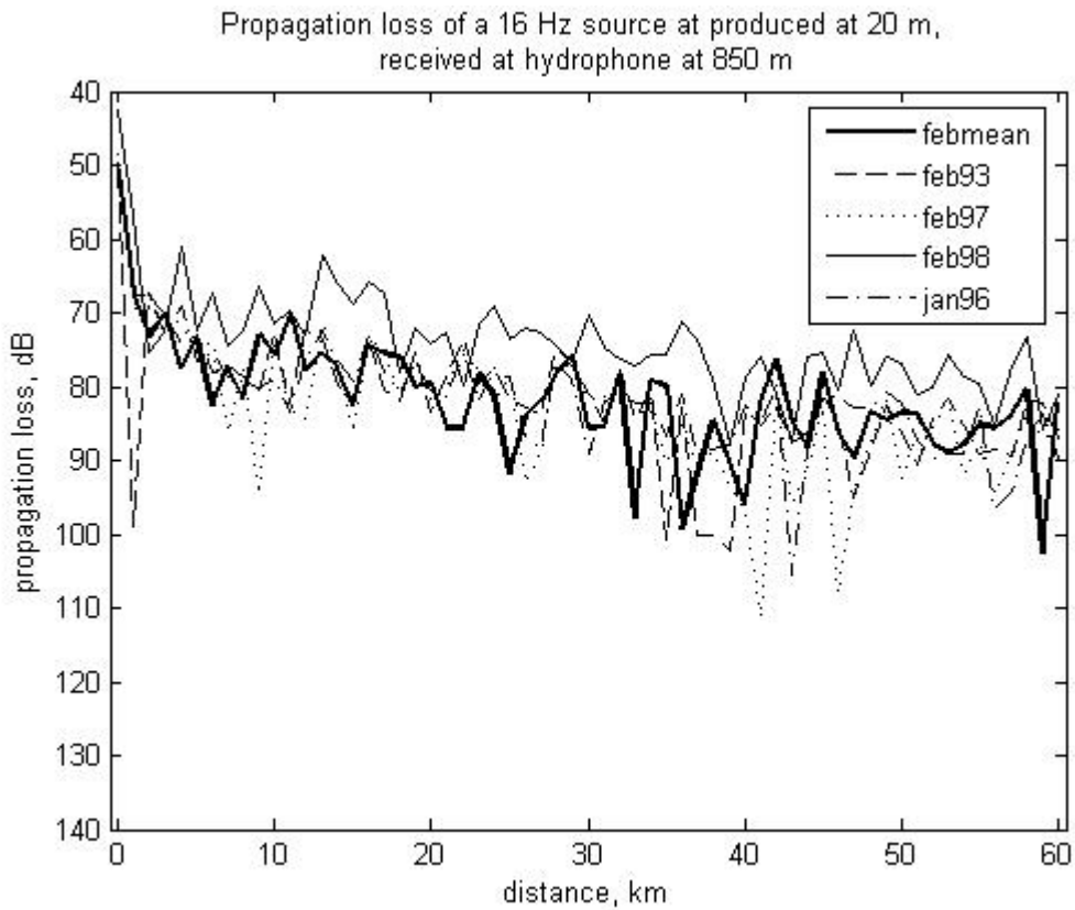
Figure 4. Transmission loss values for a blue whale B call (16 Hz) from 4 different years based on the sound speed profiles from Figure 3. Note that transmission loss is lowest during the El Niño year (solid thin black line), which rules out reduced call reception in this year as a reason for the very few call detections.
