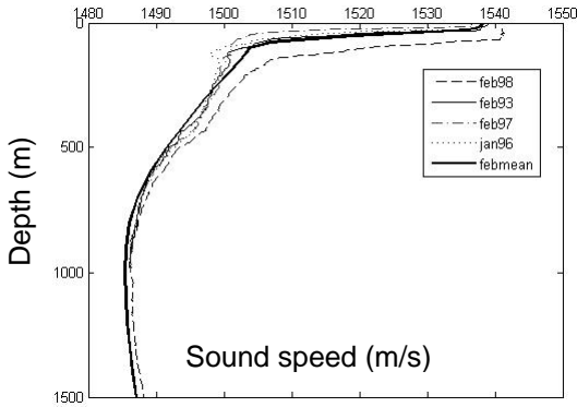
Figure 3. Sound speed profiles for February from TAO CTD casts and mean GDEM values.
