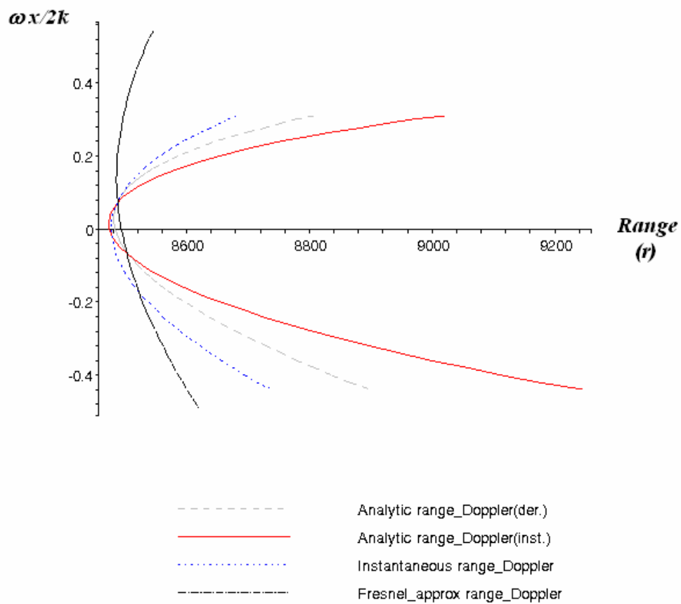
Figure 5. Slant Range-Doppler History of Point Moving Target ( \gamma_x = 0.1, \gamma_y = 0.1, \text{accel} = a = 7.1 ): Comparison
