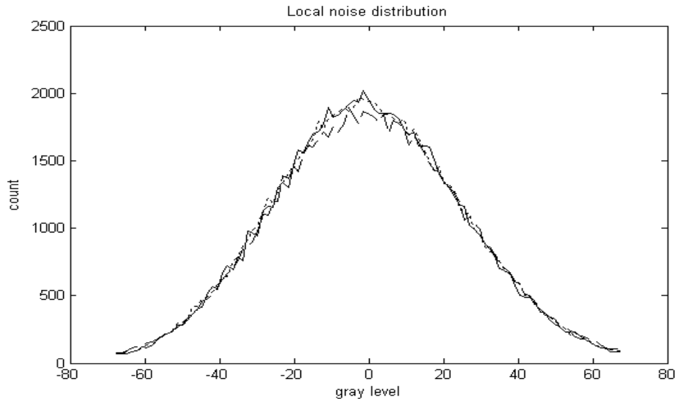
Figure 7- Distributions of the residual noise of the image acquired in satellite tracking mode (in Fig. 1). Distributions are measured at the top, middle and bottom of the image. This image was acquired by the DRDC-Ottawa SofS/CD CCD camera. The noise standard deviation is uniform over the entire image.
