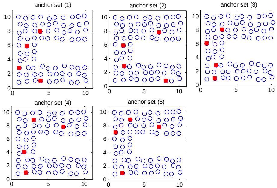
Figure 4 C-shape network scenarios with 4 anchor nodes
