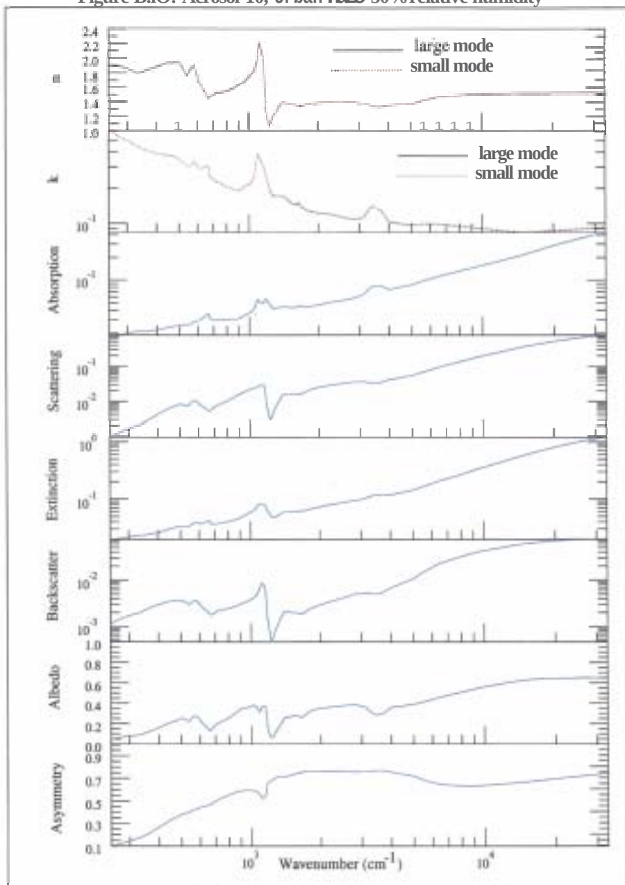
Figure B.10: Aerosol 10, Urban Haze 50% relative humidity
