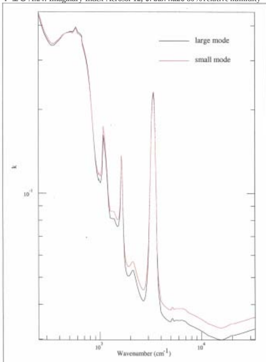
File A.24: Imaginary Index Aerosol 12, Urban Haze 80% relative humidity
