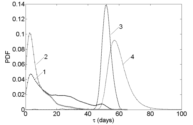
Fig. 9. \tau -PDF for the second kind of predictability (open boundary) with agiven open boundary error intensity ( \delta^2=0.2\text{ m}^2\text{ s}^{-2} ) and various tolerance levels ( \varepsilon_0^2 ): 0.005 (curve-1), 0.01 (curve-2), 0.1 (curve-3) and 0.5 (curve-4).
