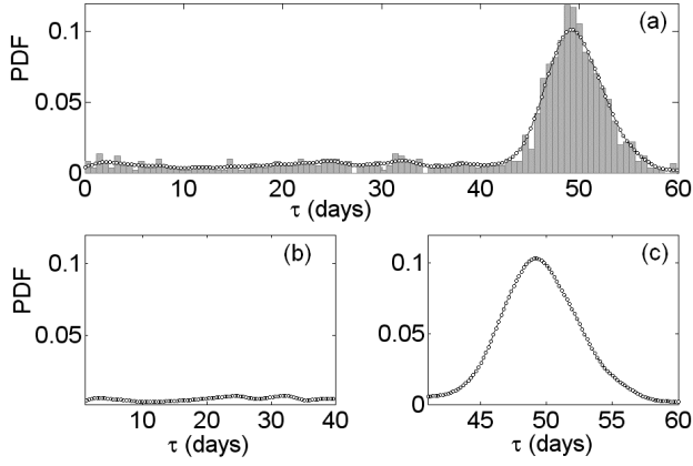
Fig. 10. “Outliers” – forecasts with \delta^2 = 0.3 \text{ m}^2 \text{ s}^{-2} , \varepsilon_0^2 = 0.1 : (a) \tau -histogram computed for the perturbed open boundary, (b) best fit to the homogeneous distribution for \tau < 40 day, and (c) best fit to Gaussian distribution for \tau > 40 day.
