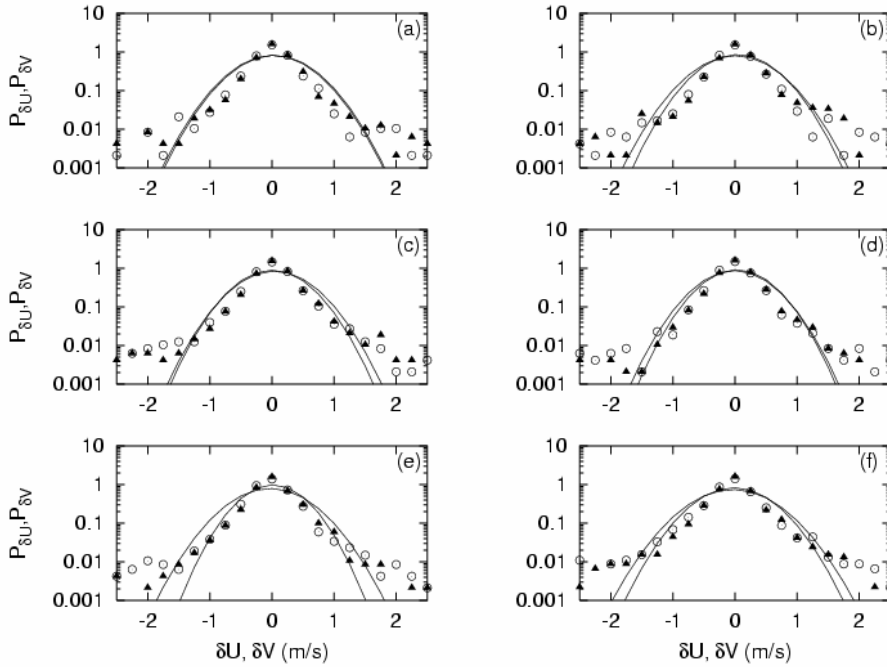
Fig. 15. P_{\delta U} = \bar{P}_2(\delta U, 0, t) (the black triangles) and P_{\delta V} = \bar{P}_2(0, \delta V, t) (the white dots) through 3 h (a), 6 h (b), 12 h (c), 24 h (d), 48 h (e) and 96 h (f). The solid lines are Gaussian approximations.
