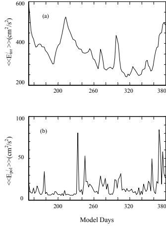
Fig. 6. Temporal evolution of \langle\langle E'_{\text{tor}} \rangle\rangle (a) and \langle\langle E'_{\text{pol}} \rangle\rangle (b).
