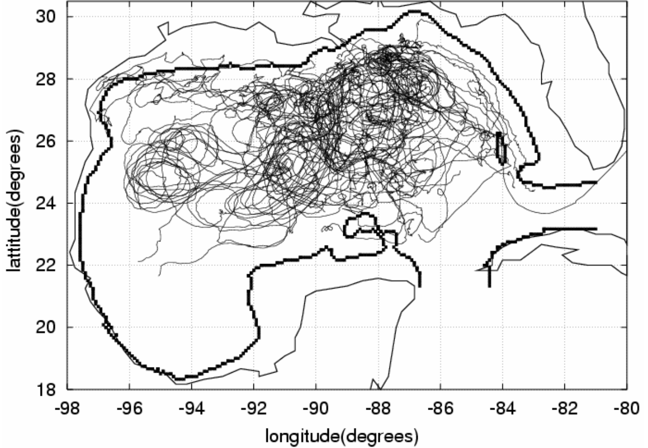
Fig. 10. Spaghetti of 55 drifting buoys used in the analysis.
