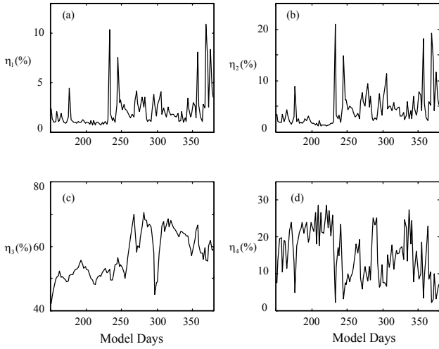
Fig. 7. Temporal evolution of non-dimensional ratios \eta_1 (a), \eta_2 (b), \eta_3 (c) and \eta_4 (d).
