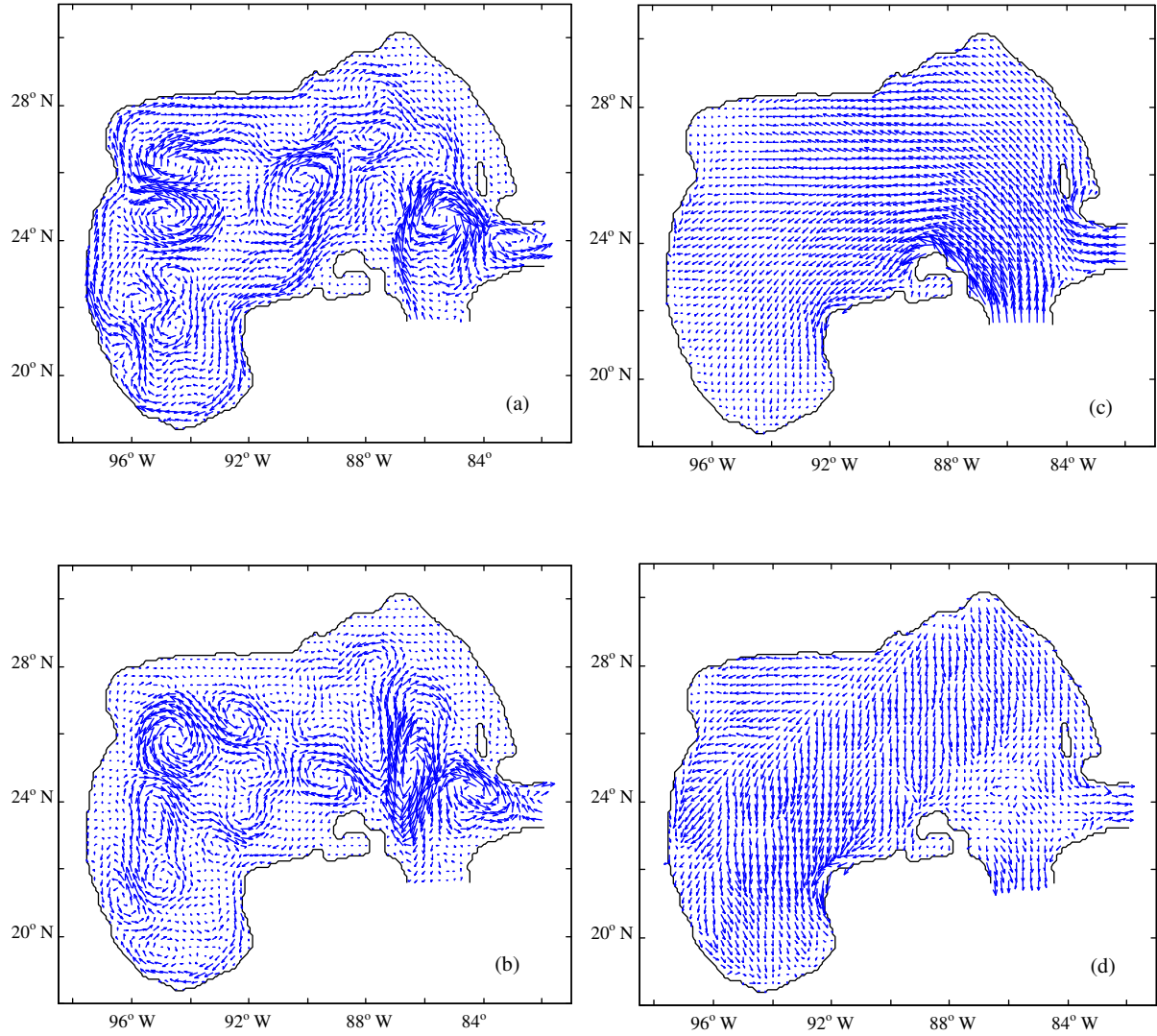
Fig. 3. Low-order toroidal [ n=1 (a), n=2 (b)] and poloidal [ m=1 (c), m=2 (d)] EOFs.
