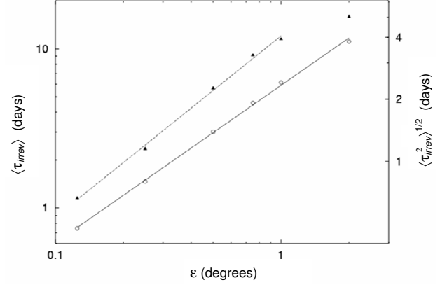
Fig. 19. The mean IT (white dots) and its variance (black triangles) as functions of the tolerance \epsilon .
