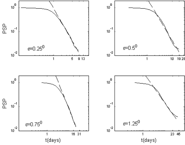
Fig. 18. PSP of IT calculated for different levels of tolerance \epsilon . Solid and dashed lines are the PSP and the proposed theoretical power laws to approximate it for large times.
