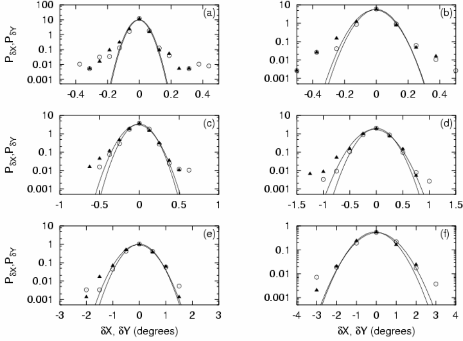
Fig. 14. P_{\delta X} = \bar{P}_1(\delta X, 0, t) (the black triangles) and P_{\delta Y} = \bar{P}_1(0, \delta Y, t) (the white dots) through 3 h (a), 6 h (b), 12 h (c), 24 h (d), 48 h (e) and 96 h (f). The solid lines are Gaussian approximations.
