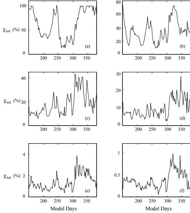
Fig. 20. RMS errors ( \chi_{\text{tor}} ) of approximation of the toroidal circulation through 1 (a), 3 (b), 6 (c), 10 (d), 30 (e) and 50 (f) toroidal EOFs.
