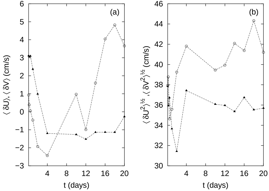
Fig. 11. Mean (a) and variance (b) of difference between buoy and particle velocities.
