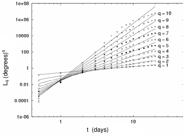
Fig. 12. The first ten moments of MPE. The solid lines represent the power laws which approximate computation results displayed by dots, crossings, triangles and squares.
