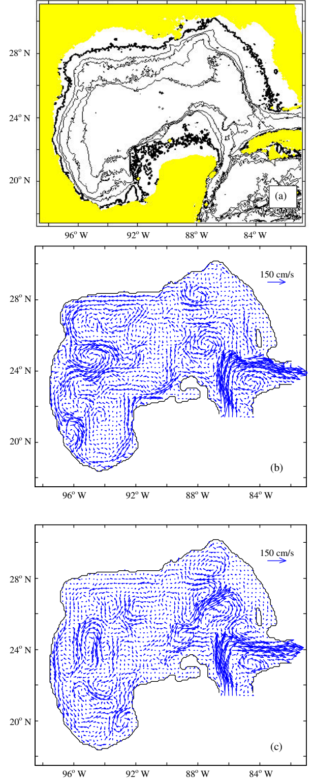
Fig. 1. High-resolution bathymetry utilized by the model (a) and circulation patterns in the Gulf of Mexico for two different dynamical regimes in 1998 on (b) Julian Day 260, and (c) Julian Day 320. The bold line in (a) is 50 m isobath. Transition from one regime to another is characterized by energy cascade from low- to high-order EOFs.
