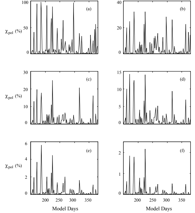
Fig. 21. RMS errors ( \chi_{\text{pol}} ) for the poloidal circulation approximated through 1 (a), 3 (b), 6 (c), 10 (d), 30 (e) and 50 (f) poloidal EOFs.
