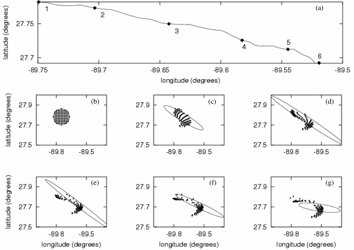
Fig. 16. Cluster spread along the trajectory (a) of H17543 drifter. Positions 1, 2, 3, 4, 5, 6 of cluster center (a) and corresponding to them positions of the cluster (b), (c), (d), (e), (f), (g) are given through every 8 h. Initially the cluster is round with the radius equaled to 1/12^\circ (b). The solid lines are the cluster boundaries predicted by the singular vector approach. The black dots are particles.
