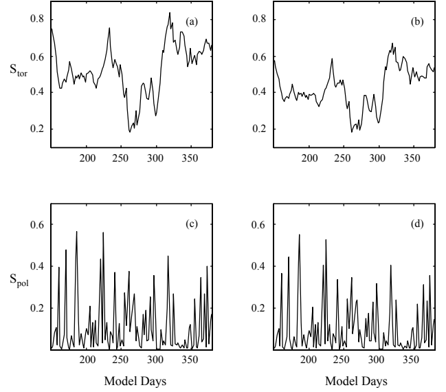
Fig. 8. Temporal behavior of the toroidal (a, b) and poloidal (c, d) entropies computed for 16 (a, c) and 50 (b, d) EOFs.
