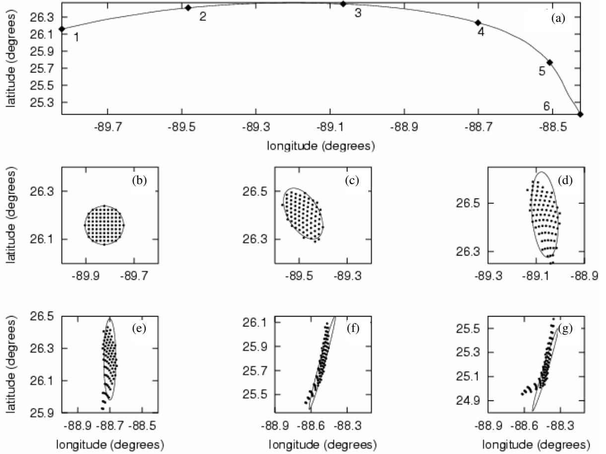
Fig. 17. Cluster spread along the trajectory (a) of H17547 drifter. Positions 1, 2, 3, 4, 5, 6 of cluster center (a) and corresponding to them positions of the cluster (b), (c), (d), (e), (f), (g) are given through every 15 h. Initially the cluster is round with the radius equaled to 1/12^\circ (b). The solid lines are the cluster boundaries predicted by the singular vector approach. The black dots are particles.
