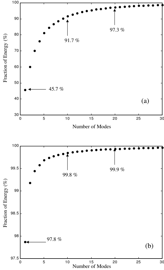
Fig. 4. The fractions of toroidal (a) and poloidal (b) energies. Arrows indicate the fraction of energy corresponding to 1, 10 and 20 EOF decomposition.
