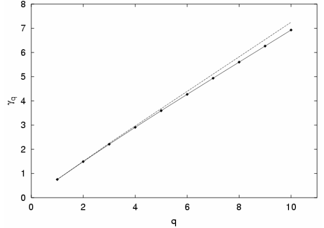
Fig. 13. The scaling exponent \gamma_q as measured within the range 12 \text{ h} < t < 20 days. Dashed line is the 3q/4 law. Solid line is the best fit. Difference between the 3q/4 law and the best fit observed for the moments numbered higher than 4 is explained by reducing accuracy of computational results from finite sampling time effects.
