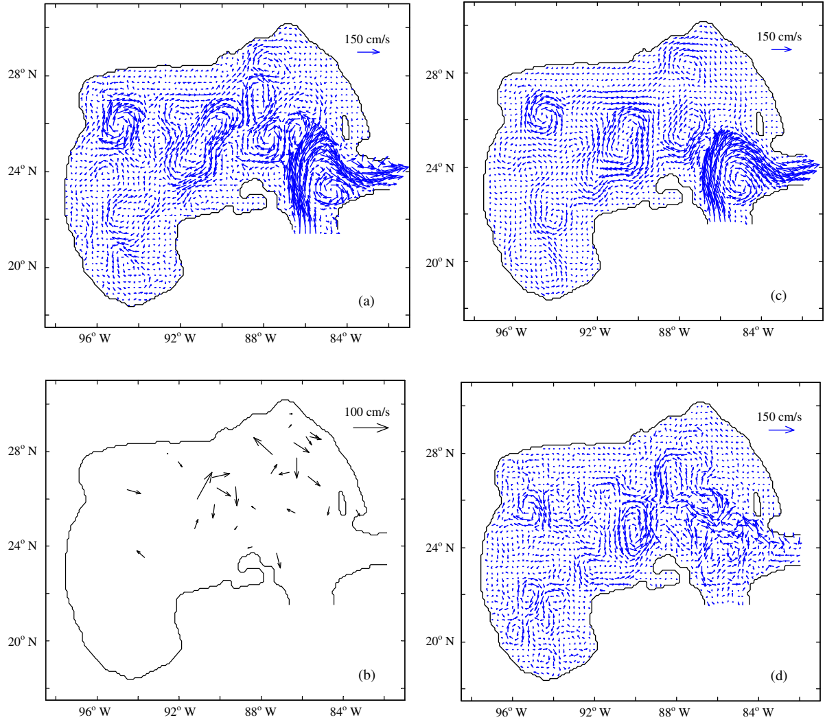
Fig. 22. Model circulation on 186 Julian Day (a), velocities calculated from the drifters for the same time (b), the reconstructed circulation (c) and the residual circulation (d).
