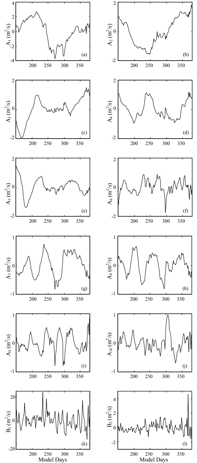
Fig. 5. Temporal evolution of mode amplitudes A_1, \dots, A_{10} at (a), ..., (j) and B_1, B_2 at (k), (l).
