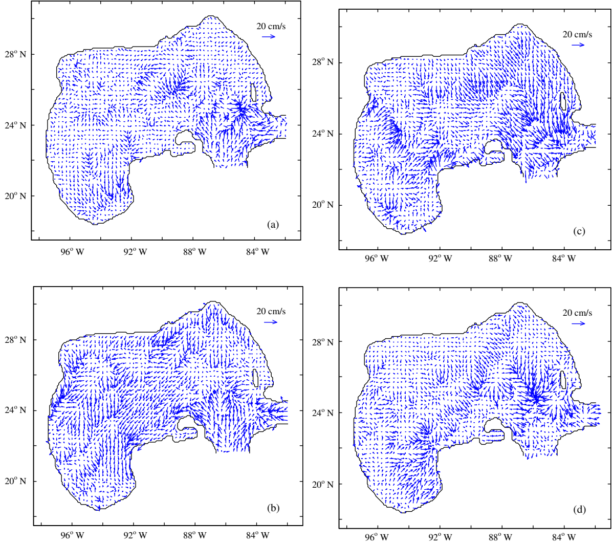
Fig. 9. Model reproduced poloidal circulation in 1998 on Julian Day 200 (a), Julian Day 235 (b), Julian Day 300 (c), and Julian Day 360 (d).
