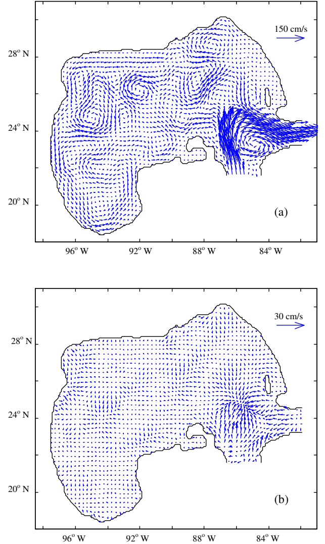
Fig. 2. Structures of the toroidal (a) and poloidal (b) SPCs.
