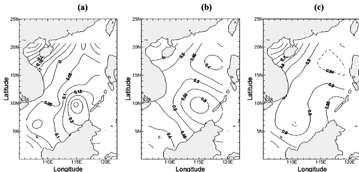
FIG. 9. Distributions of SWH (a) bias, (b) rms error, and (c) correlation coefficient between WWATCH and T/P altimeter data for the entire year of 2000.
