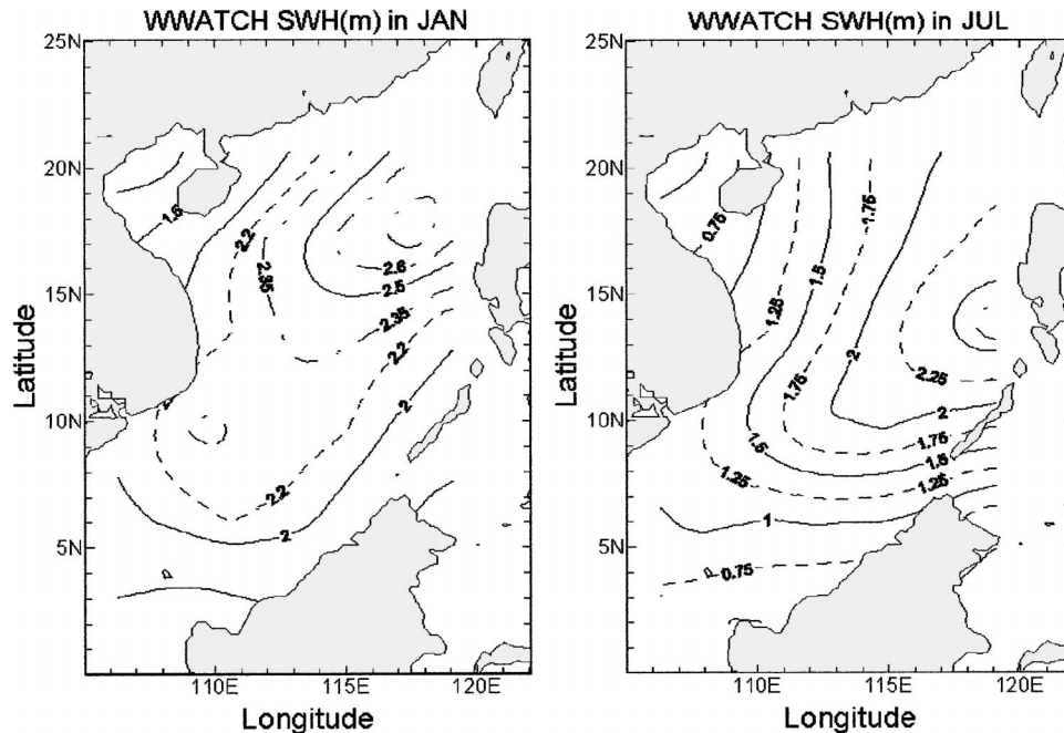
FIG. 4. Simulated monthly mean SWH using WWATCH: (a) Jan and (b) Jul 2000.
