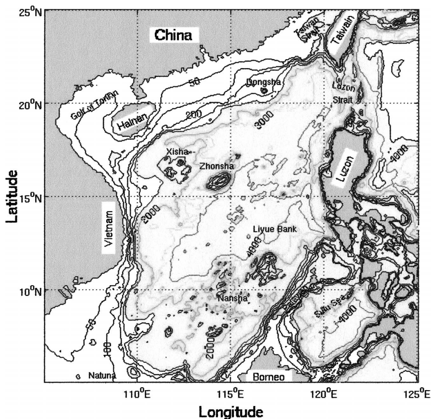
FIG. 1. Geography and isobaths showing the bottom topography of the South China Sea.
