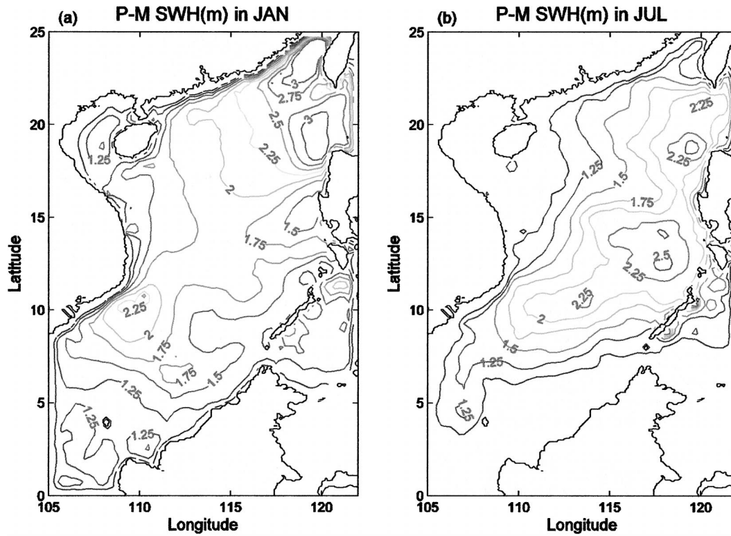
FIG. 5. Calculated monthly mean SWH using the Pierson-Moskowitz spectrum: (a) Jan and (b) Jul 2000.
