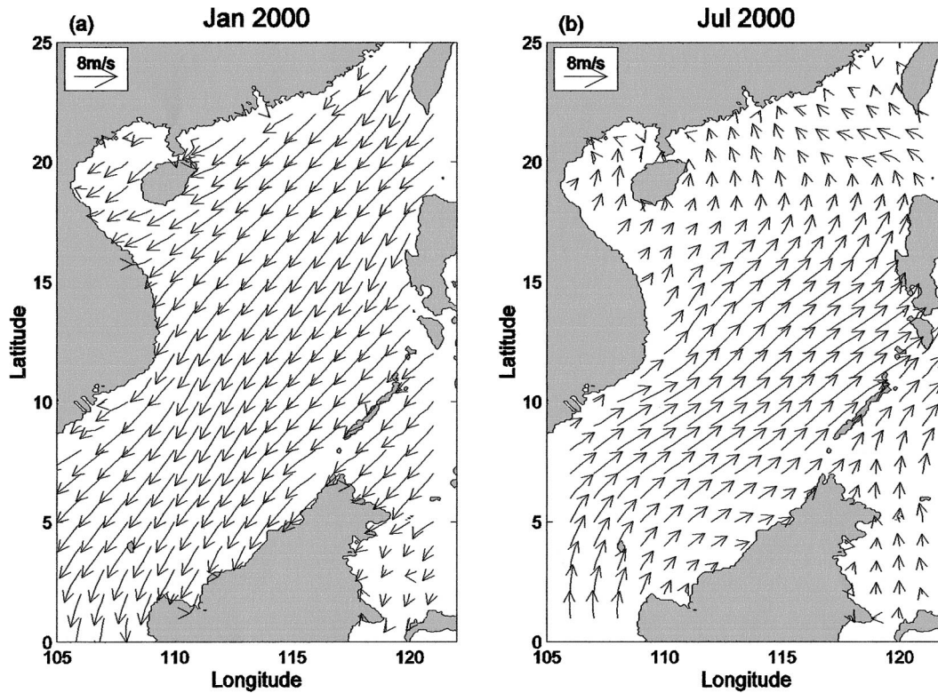
FIG. 2. Monthly mean wind speed at 10-m height computed from the QSCAT data: (a) Jan and (b) Jul 2000.
