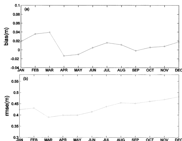
FIG. 15. Temporal evolution of (a) bias and (b) rmse for the whole SCS.
