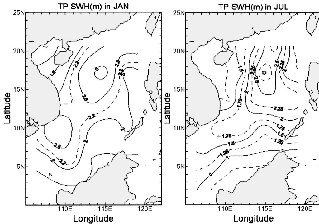
FIG. 6. Monthly mean SWH from T/P data: (a) Jan and (b) Jul 2000.
