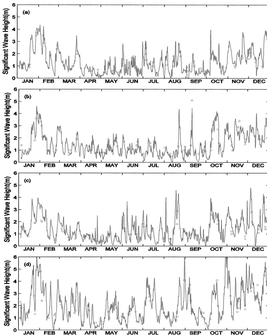
FIG. 14. Comparison between WWATCH modeled (solid curve) and T/P observed (denoted by circle) significant wave heights at (a) point 2, (b) point 6, (c) point 11, and (d) point 19.
