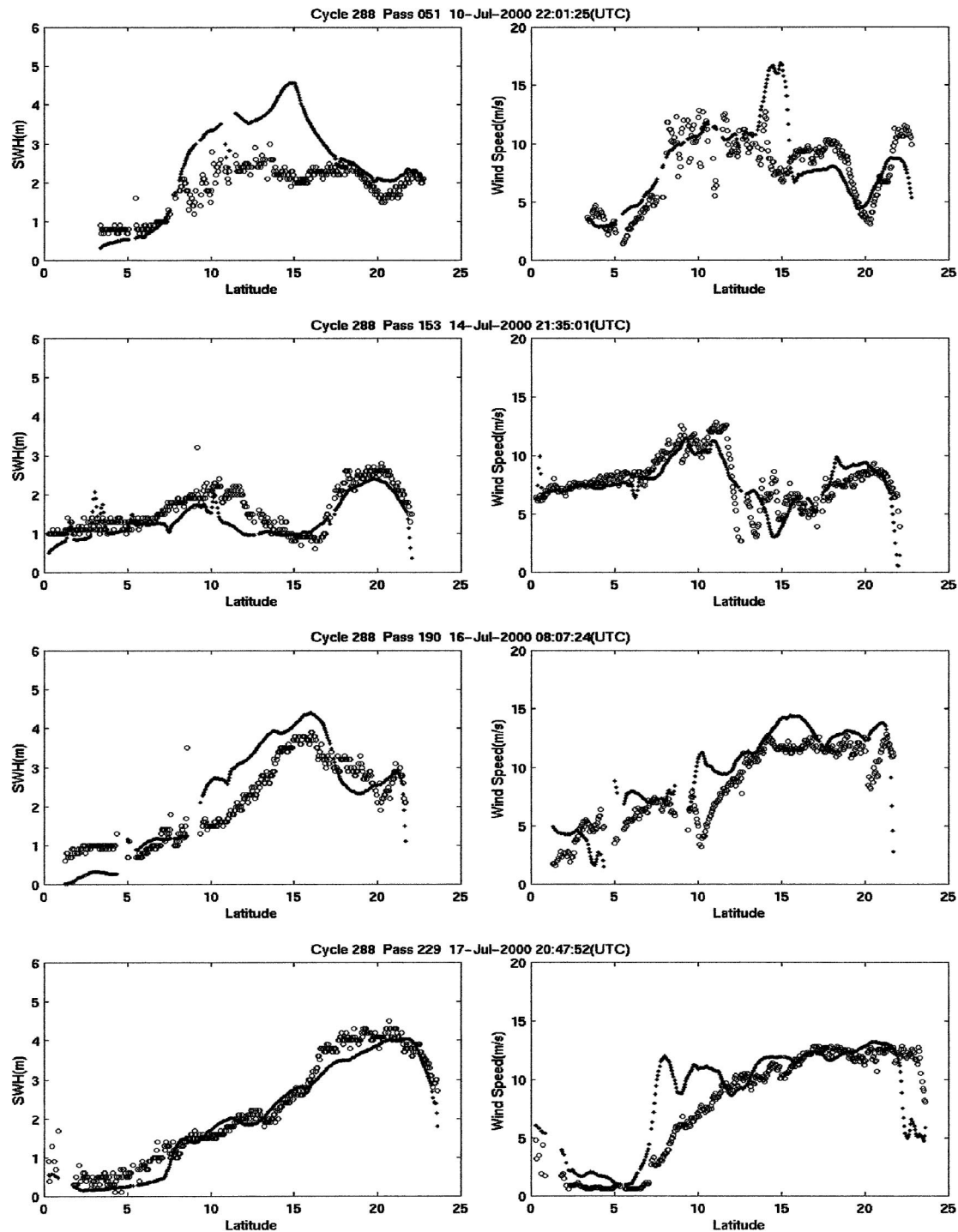
FIG. 11. Comparison between (left) modeled (dotted) and T/P observed (circle) SWHs and (right) QSCAT (dotted) and T/P observed wind speeds (circle) along the four tracks during cycle 288 (10–17 Jul 2000).
