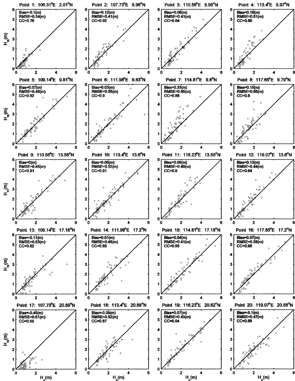
FIG. 8. Scatter diagrams of SWHs at crossover points in the SCS.
