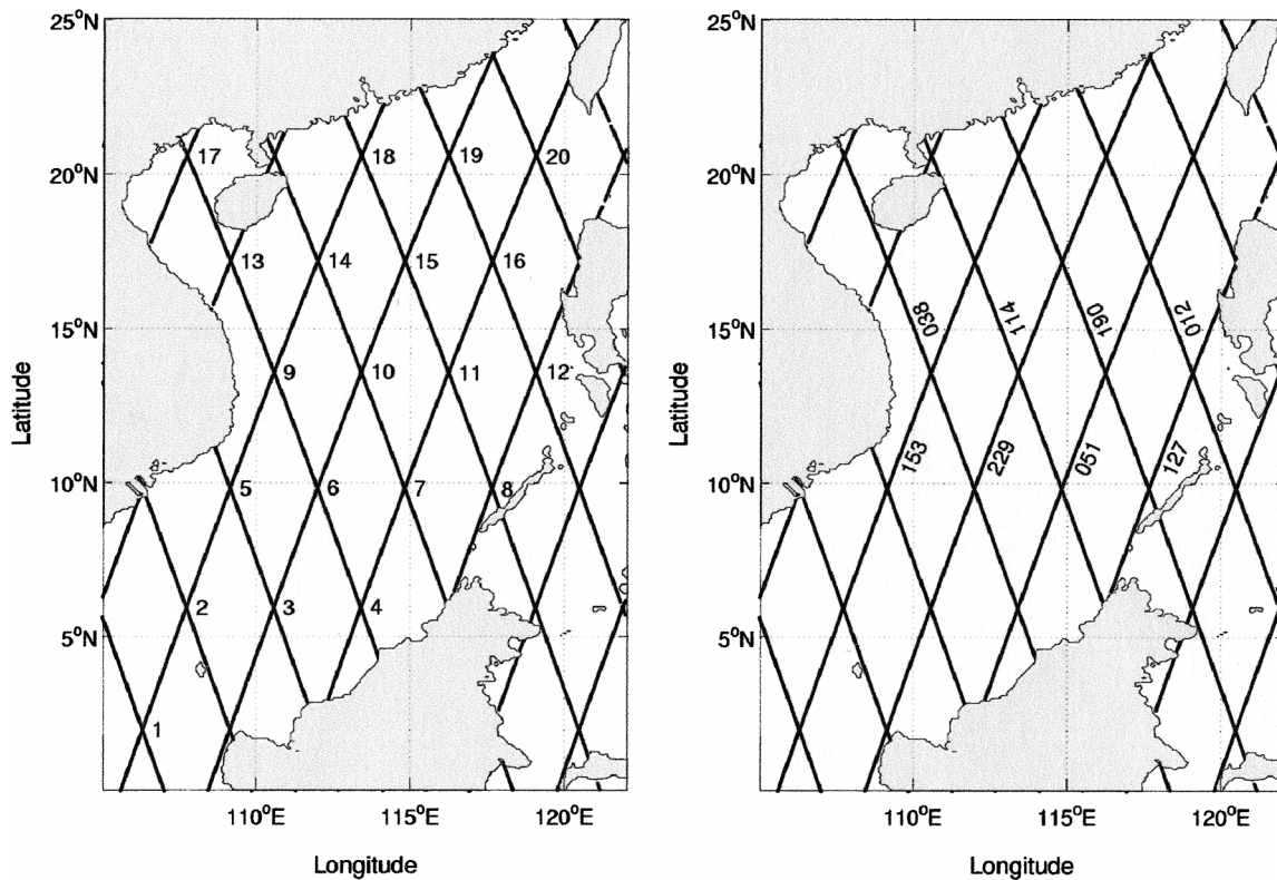
FIG. 3. The T/P satellite (a) crossover points and (b) tracks in the SCS.
