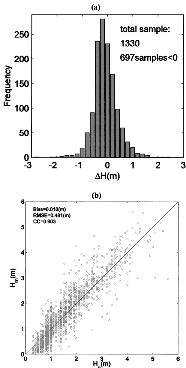
FIG. 7. Model accuracy statistics: (a) histogram of model error and (b) scatter diagram of modeled ( H_m ) and observed ( H_o ) SWH for all the crossover points.
