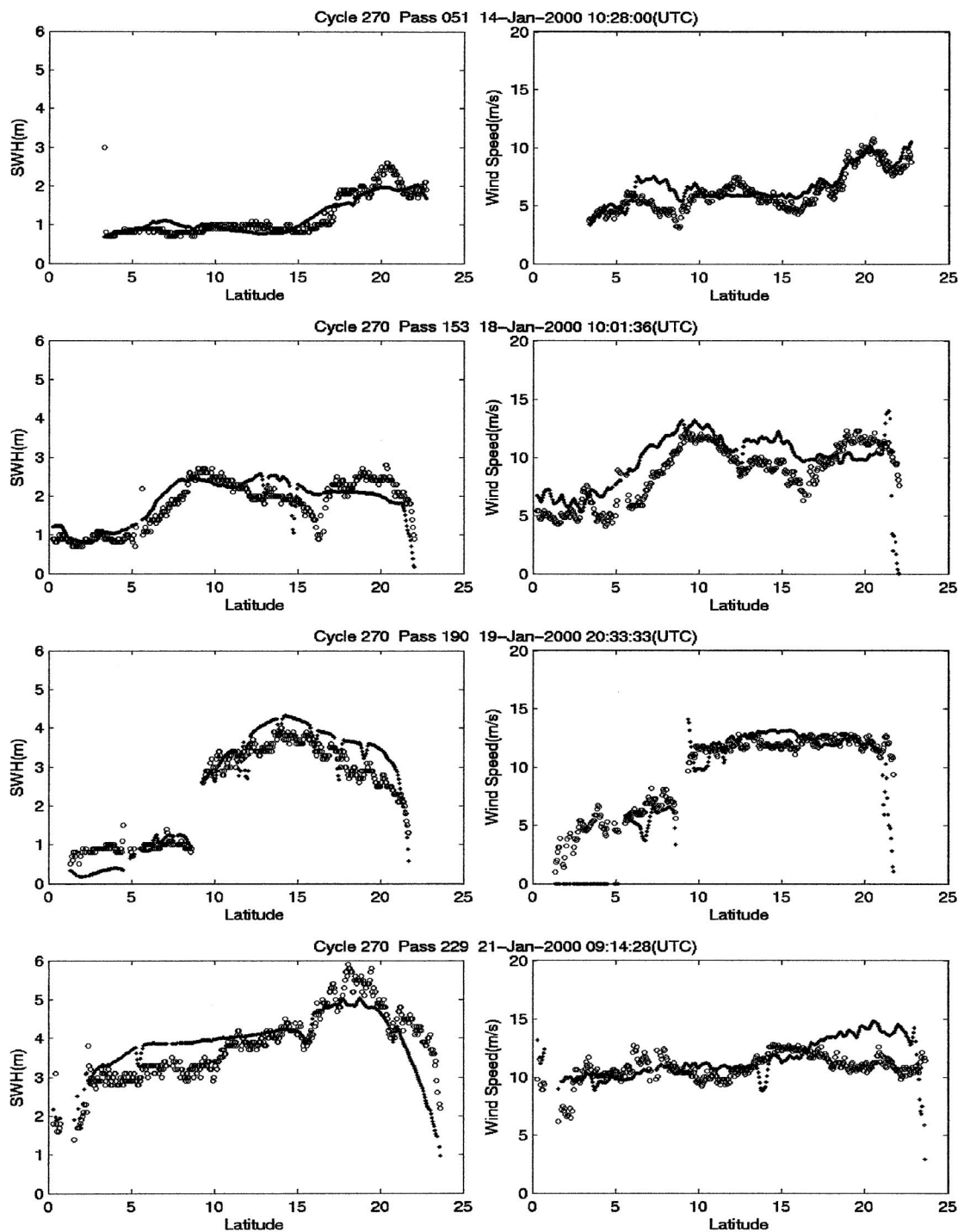
FIG. 10. Comparison between (left) modeled (dotted) and T/P observed (circle) SWHs and (right) QSCAT (dotted) and T/P observed wind speeds (circle) along the four tracks during cycle 270 (14–21 Jan 2000).
