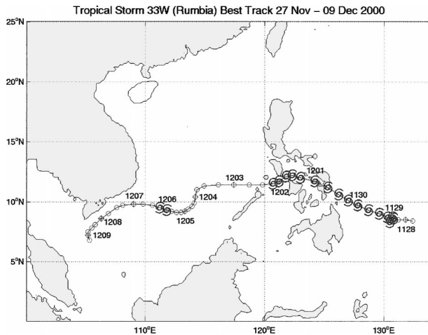
FIG. 12. Track of Tropical Storm Rumbia (2000).
