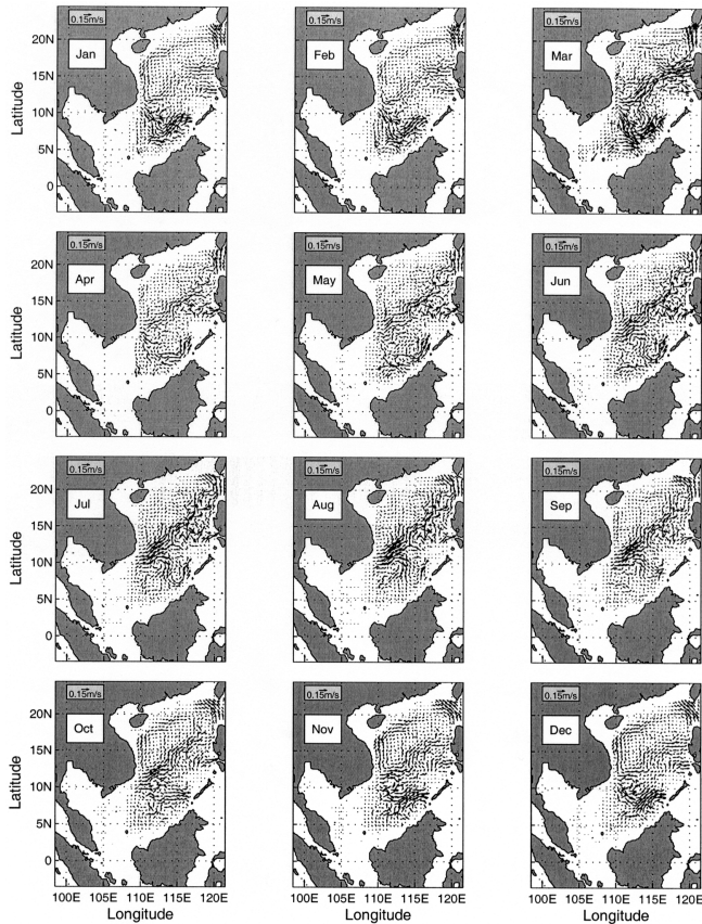
Fig. 9. Inverted monthly mean velocity field at the surface.
