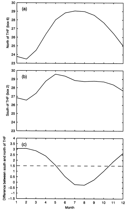
Fig. 17. Monthly evolutions of (a) SST ( ^{\circ}\text{C} ) north of THF (Box-6), (b) SST ( ^{\circ}\text{C} ) south of THF (Box-2), and (c) the difference between the two ( \Delta\text{SST} ). A criterion of \Delta\text{SST} = 1.5^{\circ}\text{C} (denoted by the dashed line) is used to represent the occurrence of THF. If \Delta\text{SST} \leq 1.5^{\circ}\text{C} , the temperature difference is not evident across THF.
