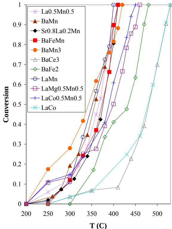
Figure 1. Light-off curves for propane combustion
