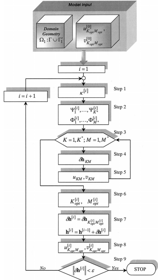
FIG. 3. Flowchart for determining the realization (\mathbf{h}^{[i]}) using the iteration process (4.2)–(4.4).
